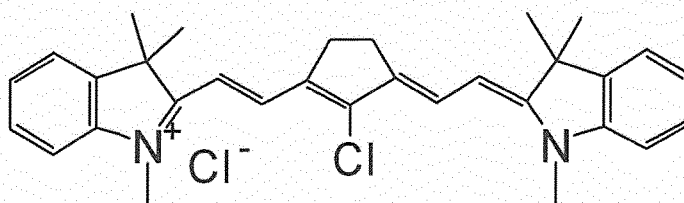
(I-x) IR797
