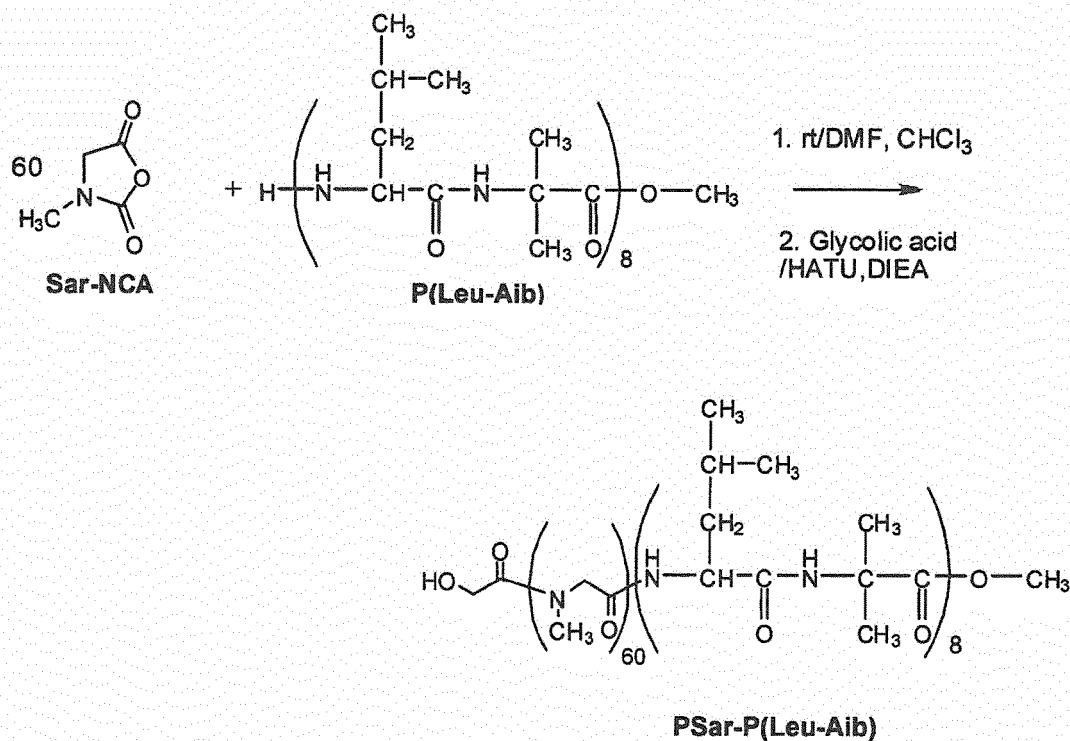
Scheme 14
