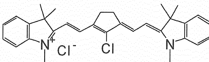
(I-x) IR797
