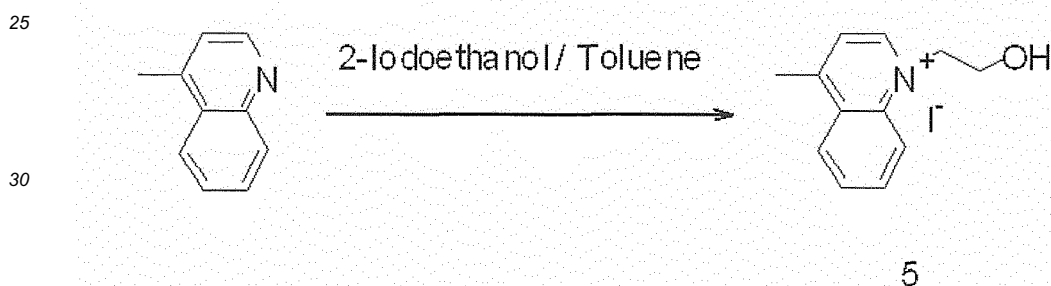
Scheme 6
