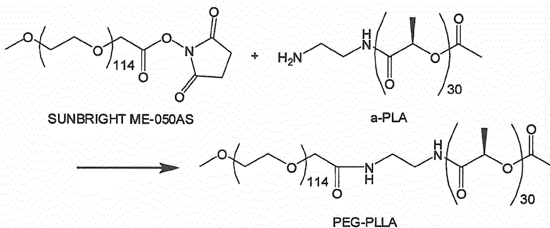
Scheme 13
