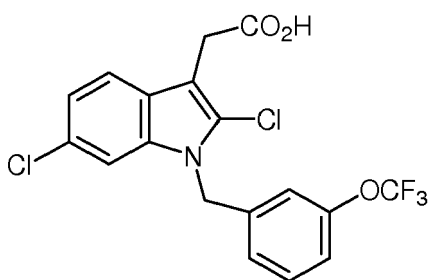
[0718] [2,5-dichloro-1-(3-trifluoromethoxybenzyl)-1H-indol-3-yl] acetic acid
