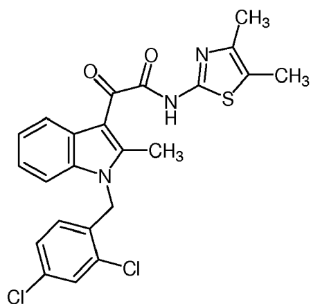
[0697] 2-[1-(2,4-dichlorobenzyl)-1 H -indol-3-yl]-N-(4,5-dimethyl-1,3-thiazol-2-yl)-2-oxoacetamide
