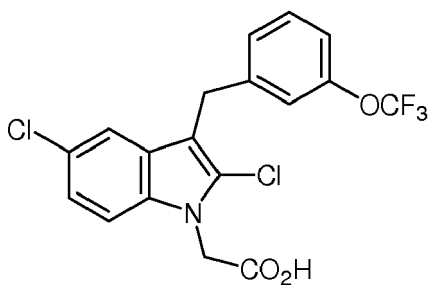
[0717] [2,6-dichloro-1-(3-trifluoromethoxybenzyl)-1H-indol-3-yl] acetic acid
