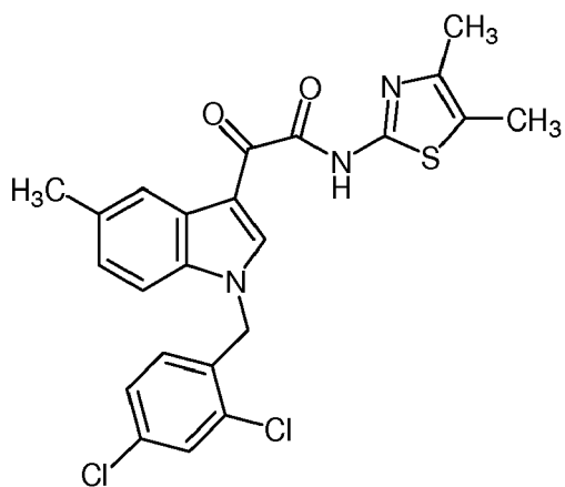
[0699] 2-[1-(2,4-dichlorobenzyl)-5-methoxy-1 H -indol-3-yl]-N-(4,5-dimethyl-1,3-thiazol-2-yl)-2-oxoacetamide
