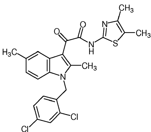
[0695] 2-[1-(2,4-dichlorobenzyl)-5-methoxy-2-methyl-1 H -indol-3-yl]- N -(4,5-dimethyl-1,3-thiazol-2-yl)-2-oxoacetamide
