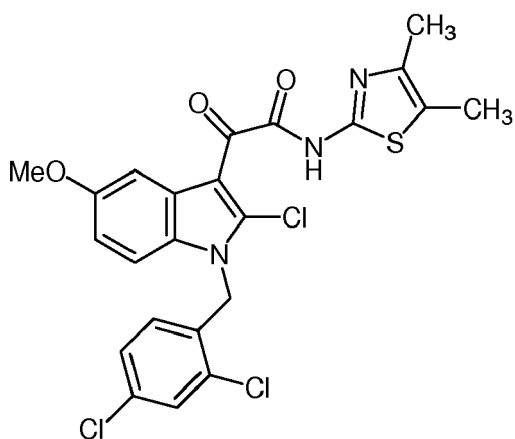
[0691] 2-[2-chloro-1-(2,4-dichlorobenzyl)-5-methyl-1 H -indol-3-yl]- N -(4,5-dimethyl-1,3-thiazol-2-yl)-2-oxoacetamide
