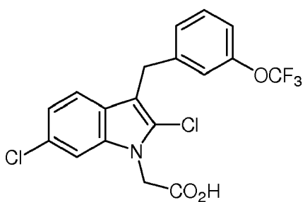
[0716] [2,5-dichloro-3-(3-trifluoromethoxybenzyl)-1H-indol-1-yl] acetic acid
