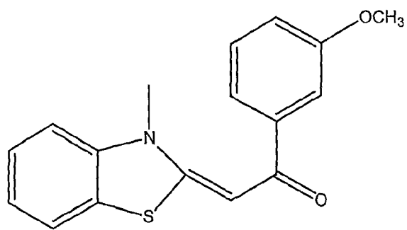
Compound 12
