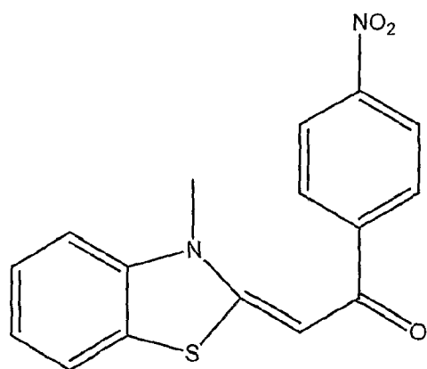
Compound 5
