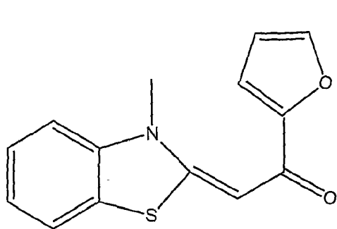
Compound 11,
