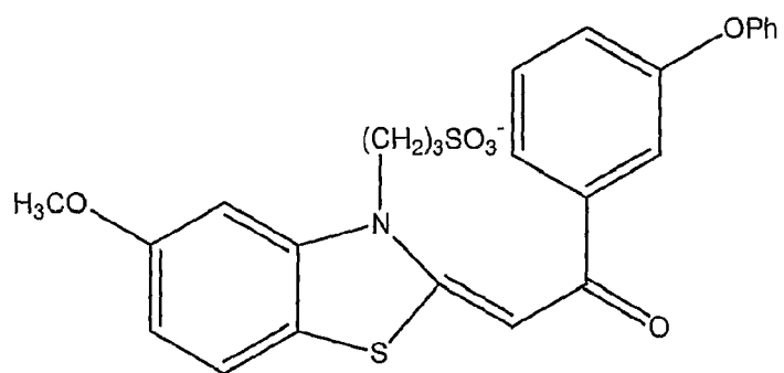
Compound 10
