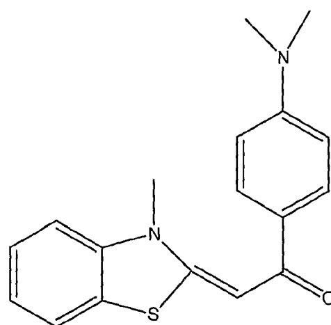
Compound 8
