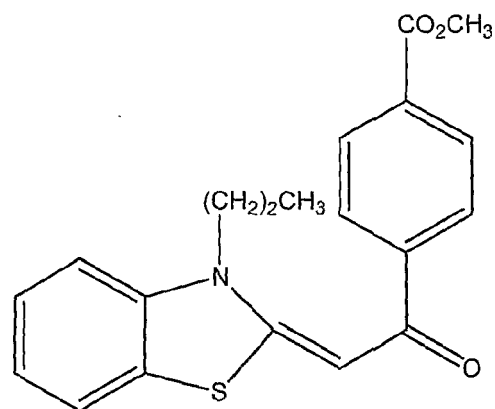
Compound 15
