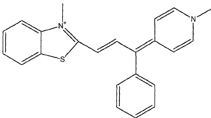
Compound 47
