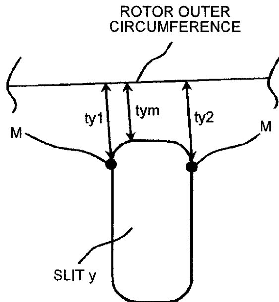
CORNERS OF SLIT y ARE ROUNDED
