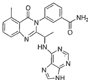
3-{5-Methyl-4-oxo-2-[1-(9H-purin-6-ylamino)-ethyl]-4H-quinazolin-3-yl}-benzamide (142)
