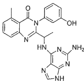
2-[1-(2-Amino-9H-purin-6-ylamino)-ethyl]-3-(3-hydroxy-phenyl)-5-methyl-3H-quinazolin-4-one (132)
