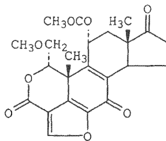
wortmannin
