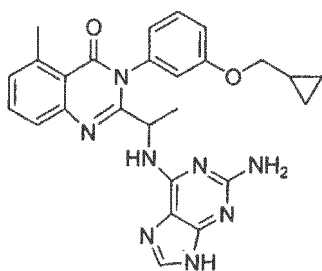
2-[1-(2-Amino-9H-purin-6-ylamino)-ethyl]-3-(3-cyclopropylmethoxy-phenyl)-5-methyl-3H-quinazolin-4-one (135)
