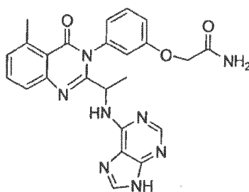
2-(3-{5-Methyl-4-oxo-2-[1-(9H-purin-6-ylamino)-ethyl]-4H-quinazolin-3-yl}-phenoxy)-acetamide (145)
