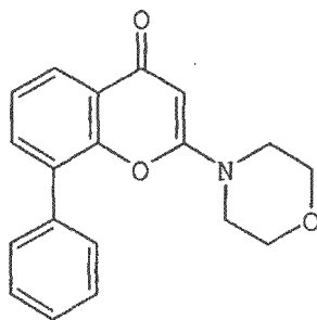
LY294002
