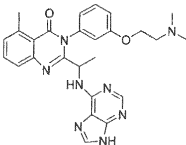
3-[3-(2-Dimethylamino-ethoxy)-phenyl]-5-methyl-2-[1-(9H-purin-6-ylamino)-ethyl]-3H-quinazolin-4-one (129)
