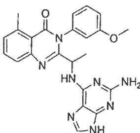
2-[1-(2-Amino-9H-purin-6-ylamino)-ethyl]-3-(3-methoxy-phenyl)-5-methyl-3H-quinazolin-4-one (134)
