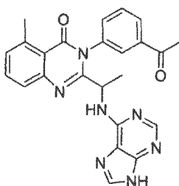
3-(3-Acetyl-phenyl)-5-methyl-2-[1-(9H-purin-6-ylamino)-ethyl]-3H-quinazolin-4-one (144)
