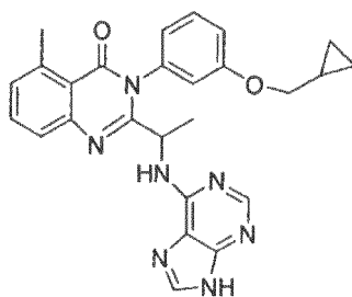
3-(3-Cyclopropylmethoxy-phenyl)-5-methyl-2-[1-(9H-purin-6-ylamino)-ethyl]-3H-quinazolin-4-one (130)
