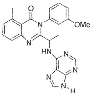
3-(3-Methoxy-phenyl)-5-methyl-2-[1-(9H-purin-6-ylamino)-ethyl]-3H-quinazolin-4-one (128)
