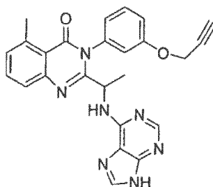
5-Methyl-3-(3-prop-2-ynyloxy-phenyl)-2-[1-(9H-purin-6-ylamino)-ethyl]-3H-quinazolin-4-one (131)
