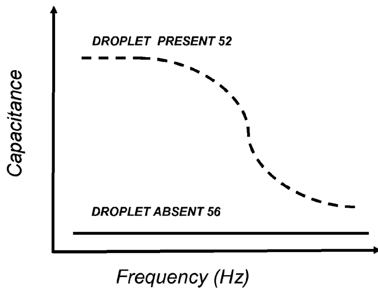
FIGURE 10: PRIOR ART
