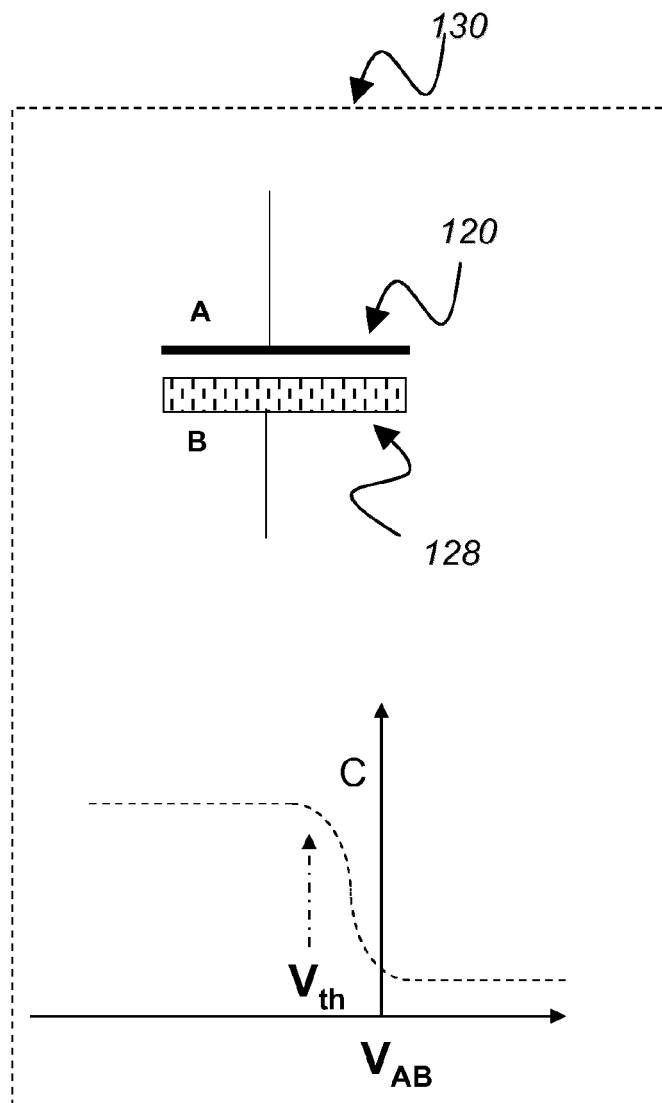
FIGURE 18: PRIOR ART
