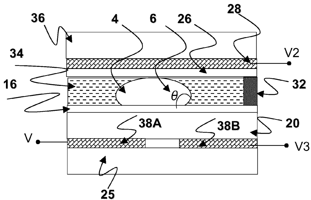
FIGURE 6: PRIOR ART
