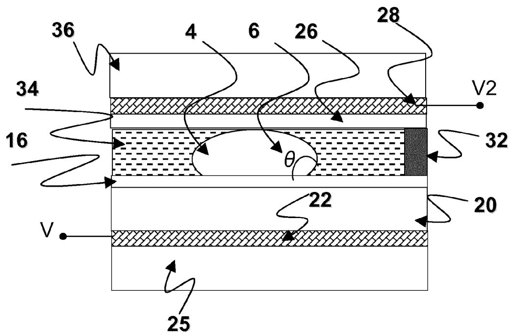
FIGURE 5: PRIOR ART
