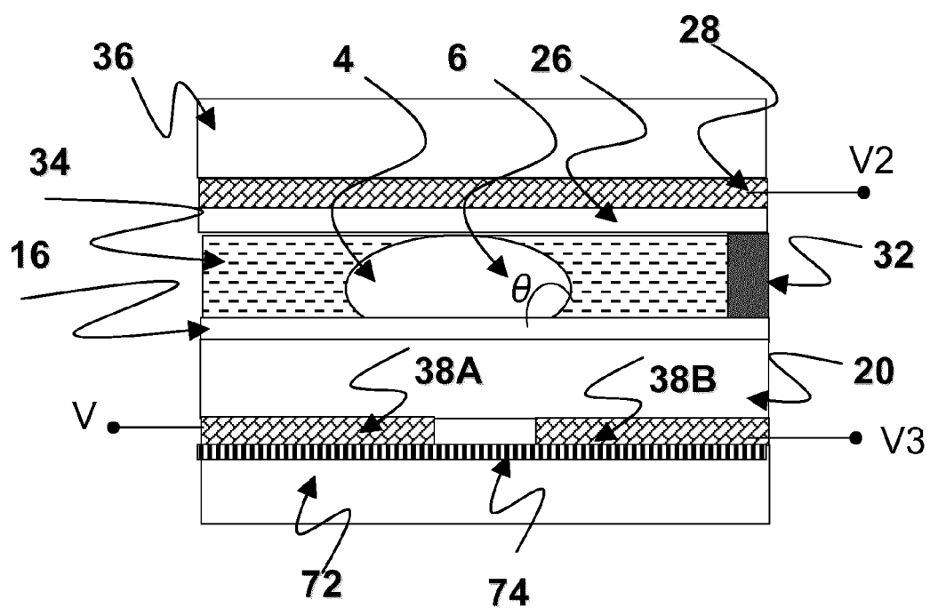
FIGURE 12: PRIOR ART
