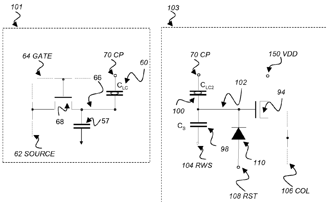
FIGURE 15: PRIOR ART
