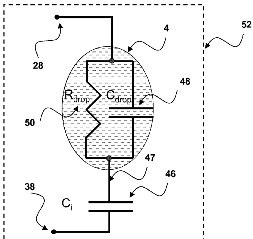
FIGURE 8: PRIOR ART
