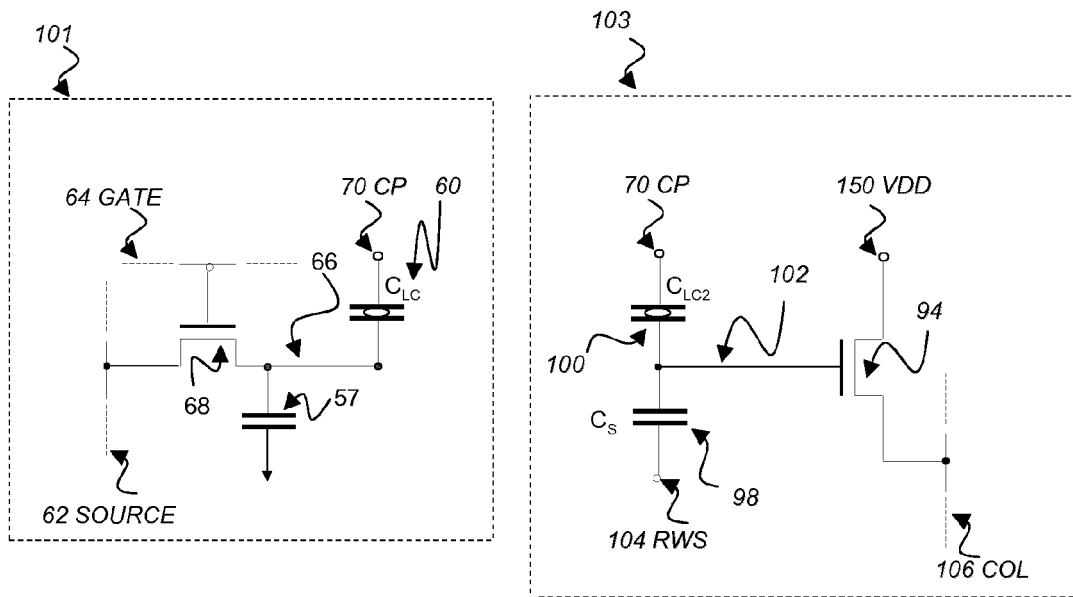
FIGURE 15: PRIOR ART
