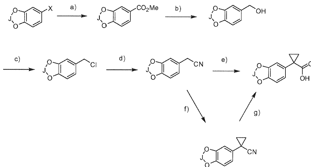
Scheme I. Preparation of cyclopropyl acids
