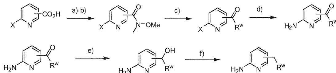
Scheme II. Preparation of amino pyridyl building blocks
