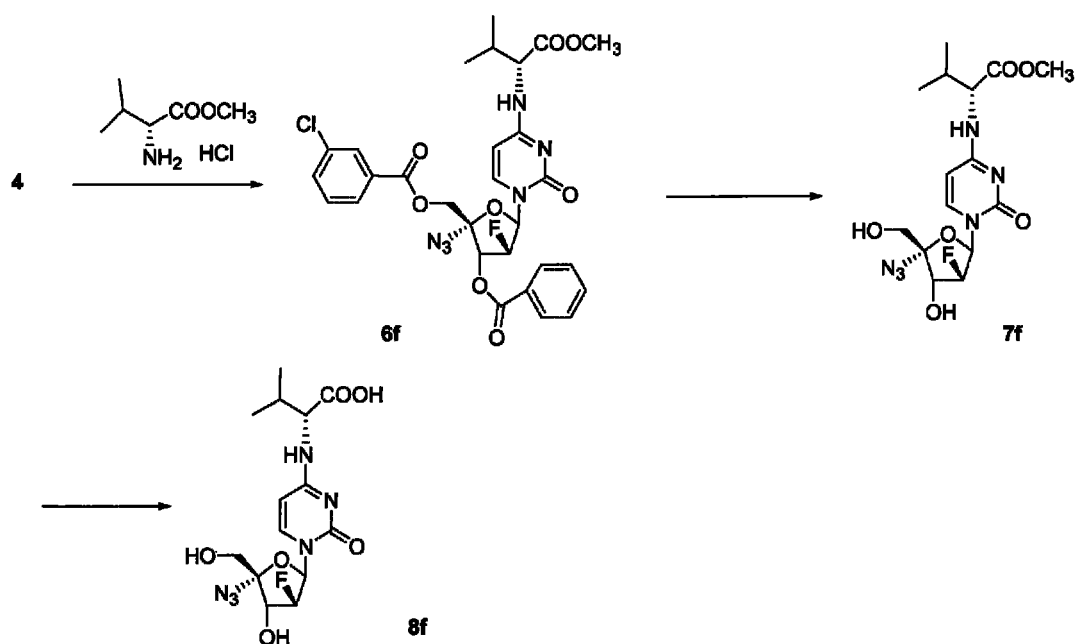
Scheme I. Synthesis of a pyrimidine nucleoside derivative with amino acid substitution at position 4.
