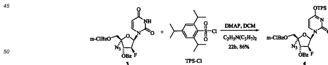
Scheme B. Synthesis of an active intermediate
