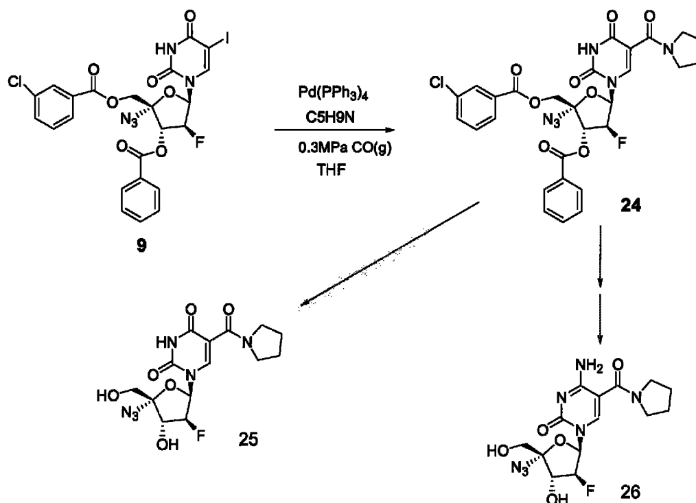
Scheme V. Synthesis of a pyrimidine nucleoside derivative with amidation at position 5.
