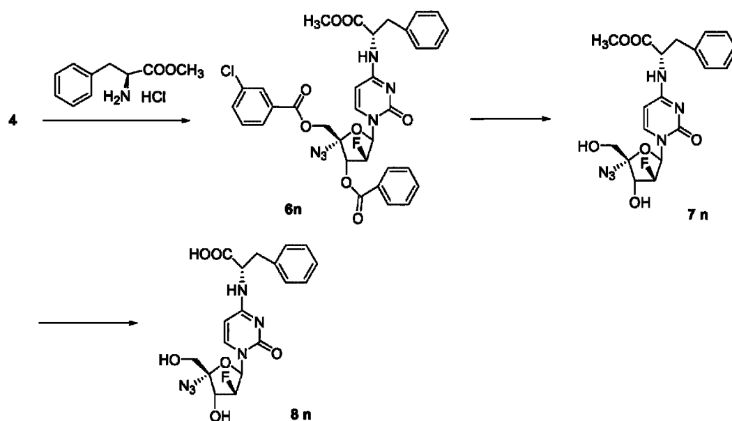
Scheme Q. Synthesis of a pyrimidine nucleoside derivative with amino acid substitution at position 4.
