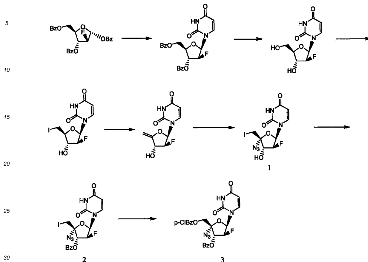
Scheme A. Synthesis of the key intermediate 3
