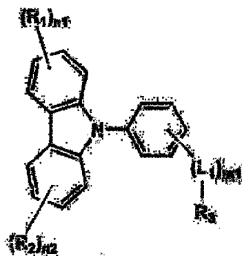
Formula (2)
