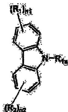
Formula (1)
