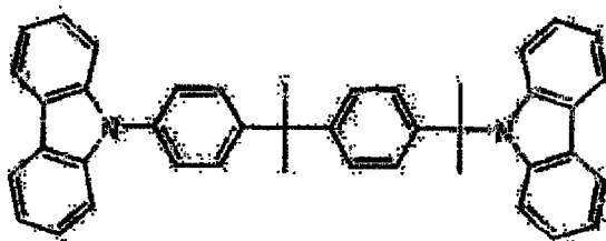
H-15
