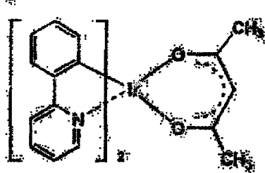
Ir-8
