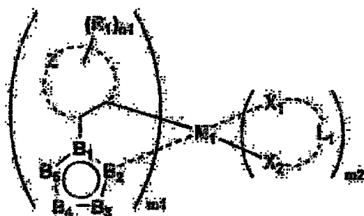
Formula (A)
