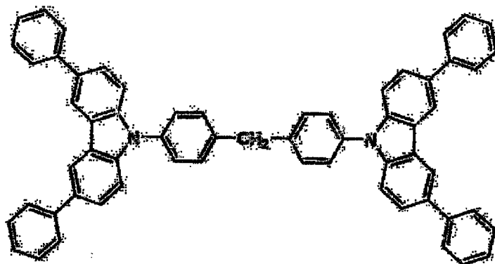
H-16
