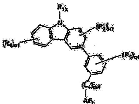
Formula (6)
