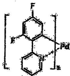
Pd-2
