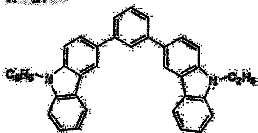
H-21
