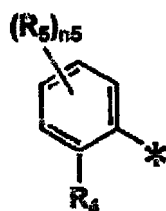
Formula (C)
