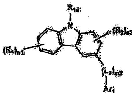
Formula (5)
