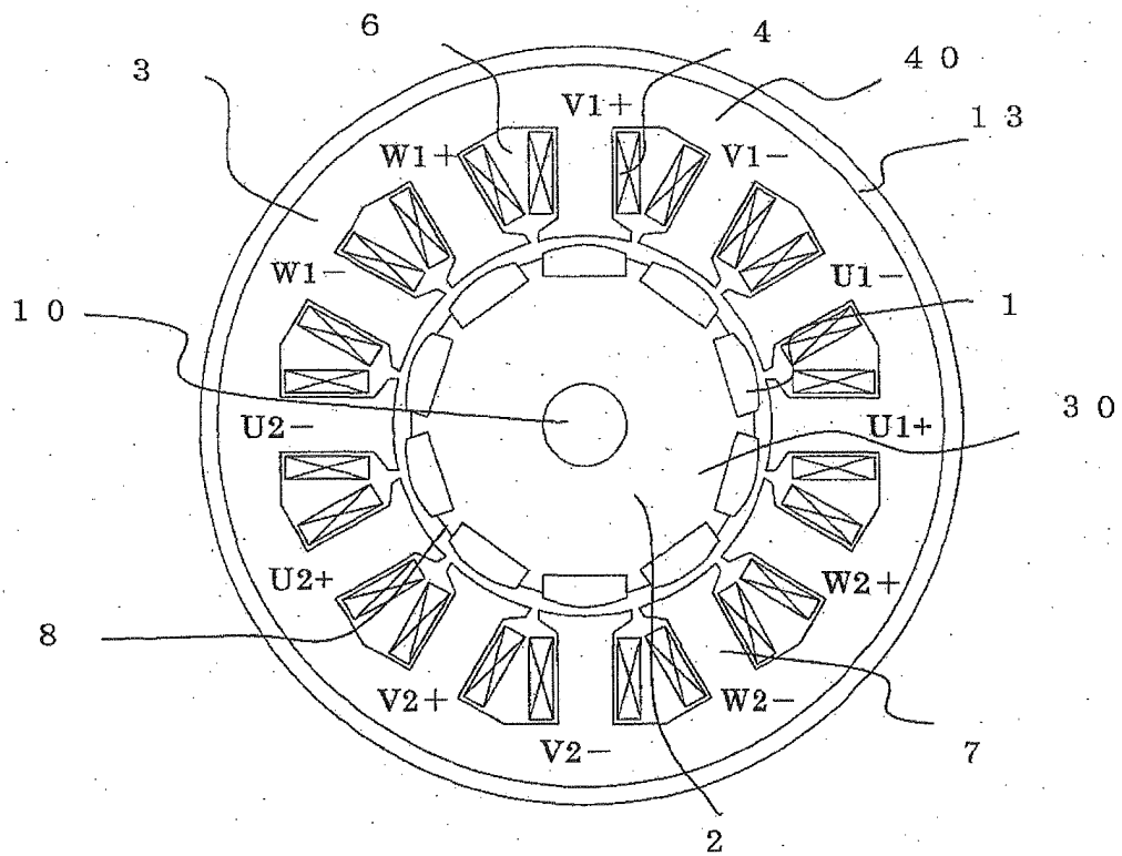
A1-A2 cross-section
