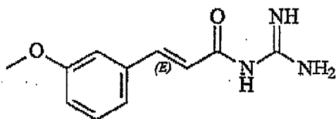
(3-Chlorocinnamoyl)guanidine comprising the structure
