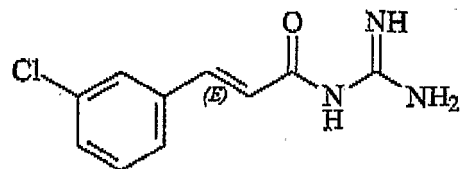
(2-Chlorocinnamoyl)guanidine comprising the structure
