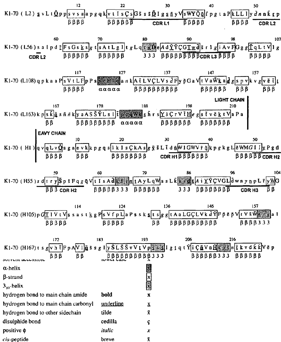
Figure 9a Representation of K1-70 Fab structure in JOY format
