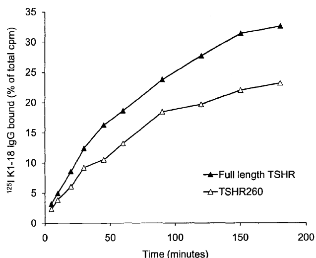
Figure 1j Time course of binding of 125 I-labelled K1-18 IgG to full length TSHR and TSHR260 coated tubes
