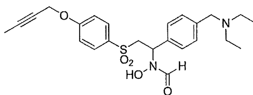
(I-1)
