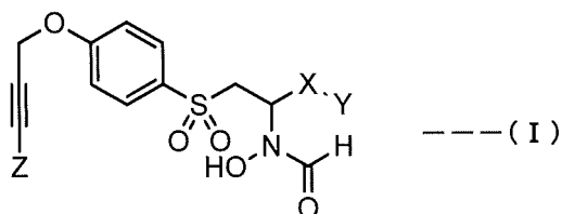
[Chem. 9]
