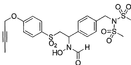
(I-19)
