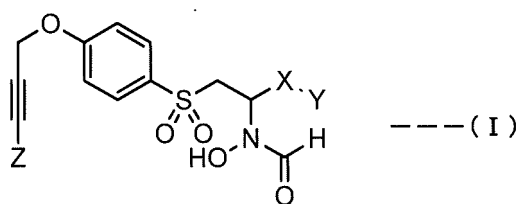
[Chem. 7]
