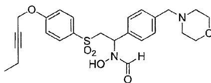
(I-7)
