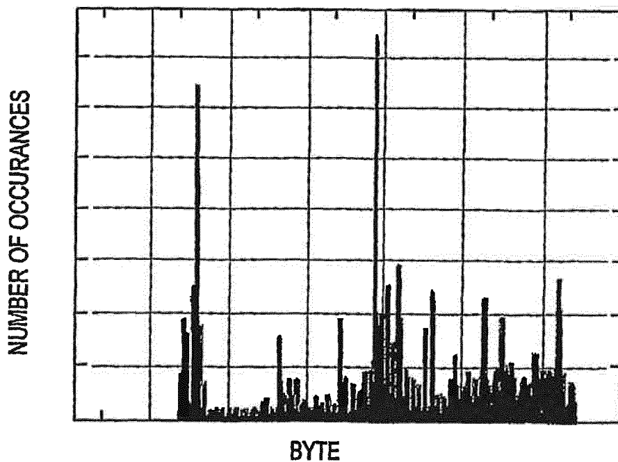
MODEL DLL
