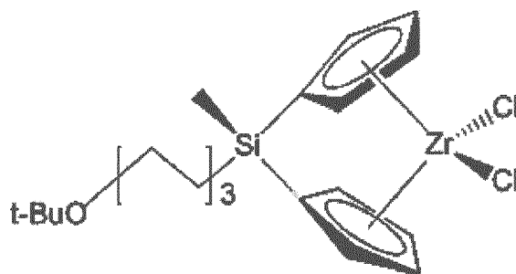
[Chemical Formula 4]
