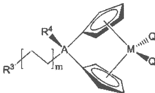
[Chemical Formula 2]
