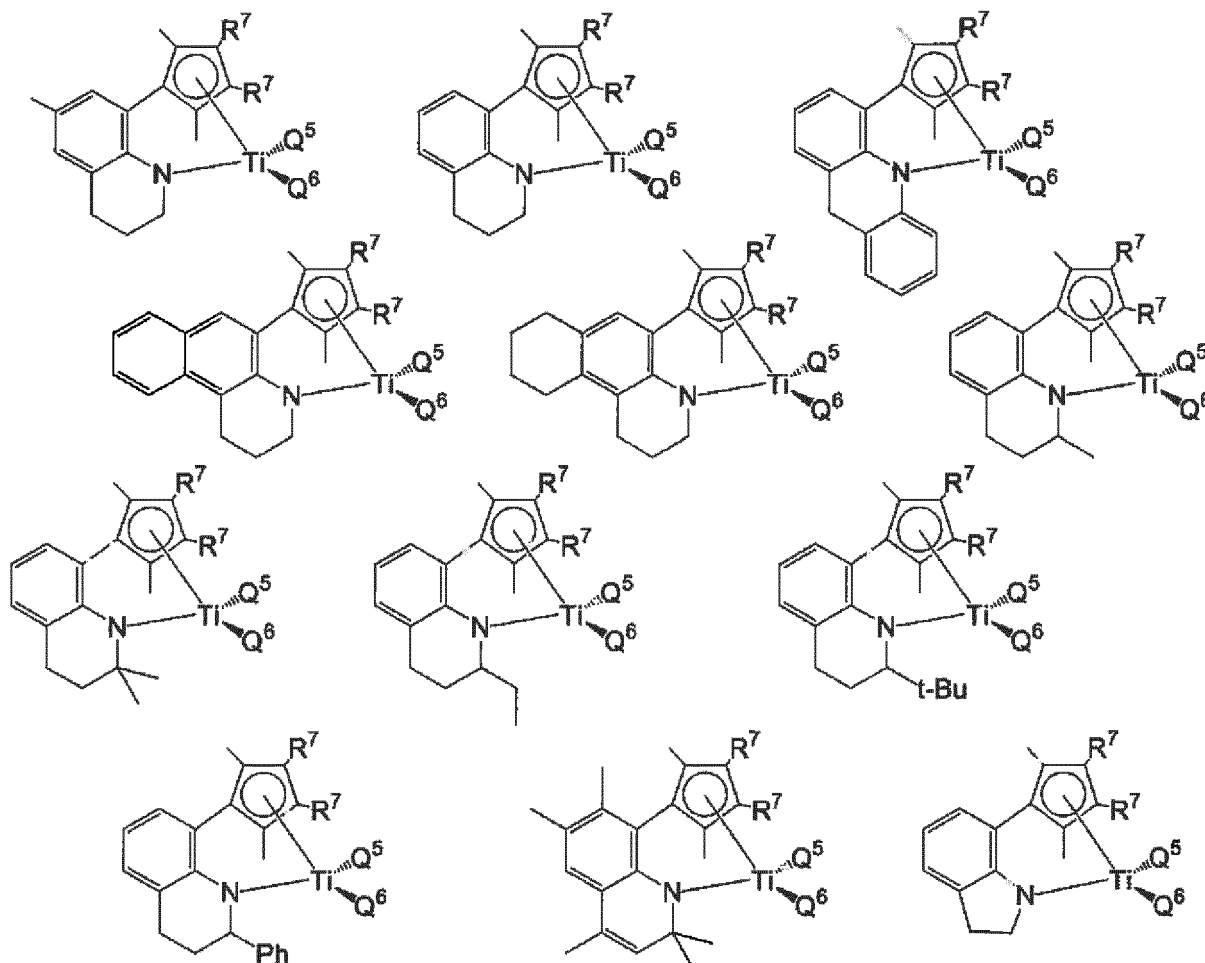
[Chemical Formula 7]
