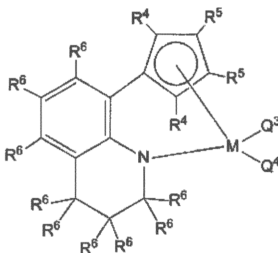
[Chemical Formula 6]
