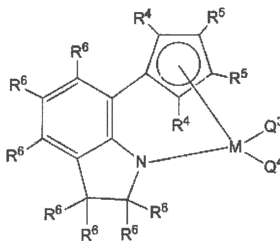
[Chemical Formula 6]
