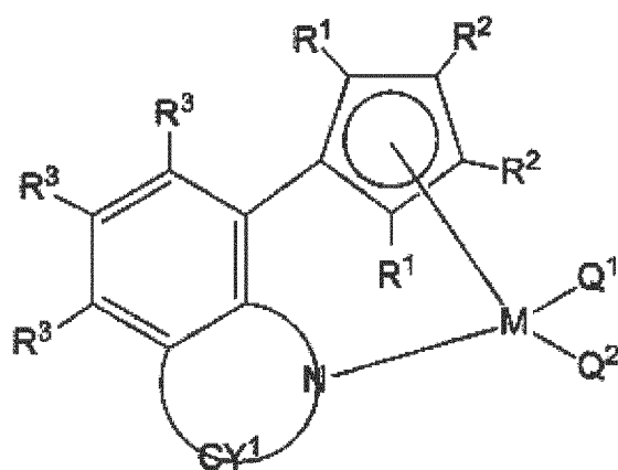
[Chemical Formula 3]
