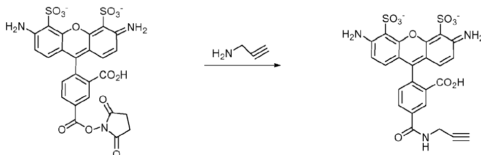
Compound 1
