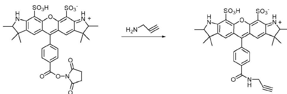
Compound 2
