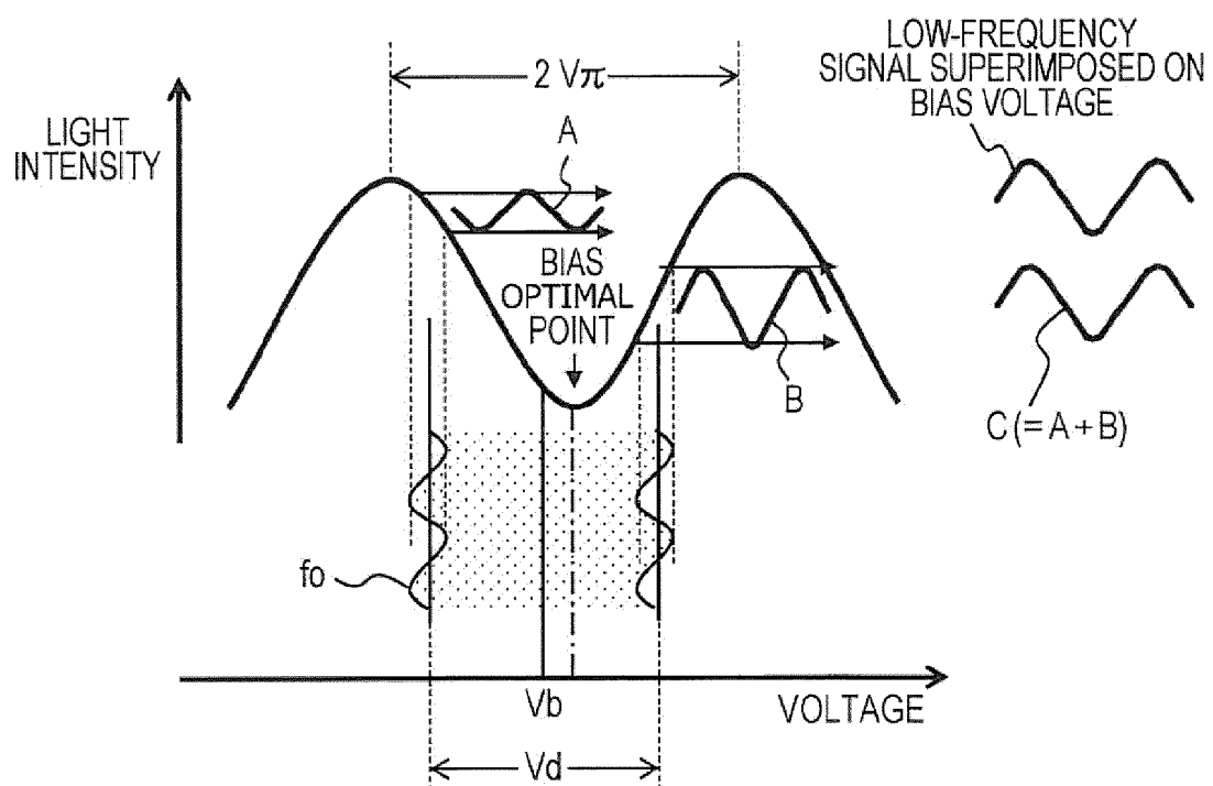
FIG. 3 RELATED ART
