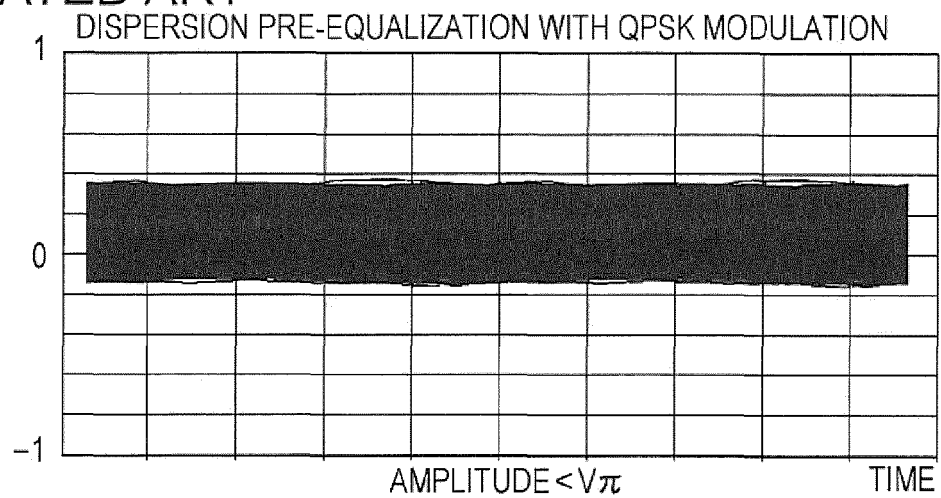
FIG. 2C RELATED ART
