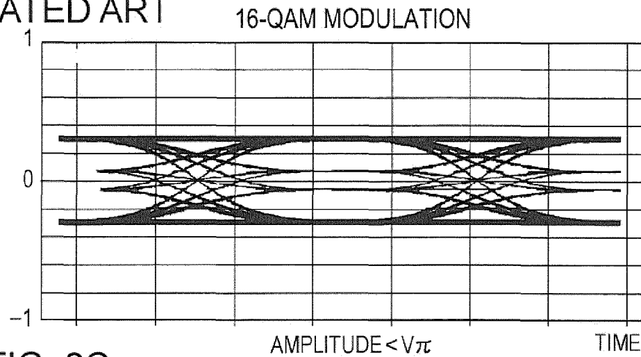
FIG. 2C RELATED ART
