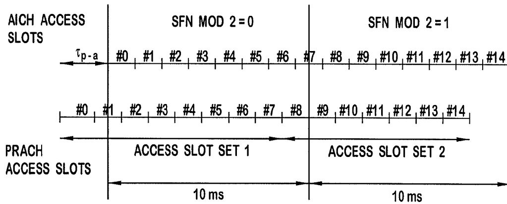
FIG. 2 (PRIOR ART)
