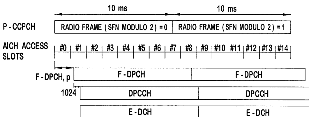
FIG. 4 (PRIOR ART)
