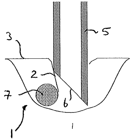
FIGURE 4 (PRIOR ART)
