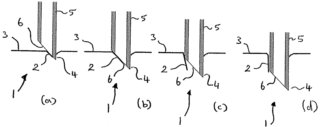
FIGURE 1 (PRIOR ART)
