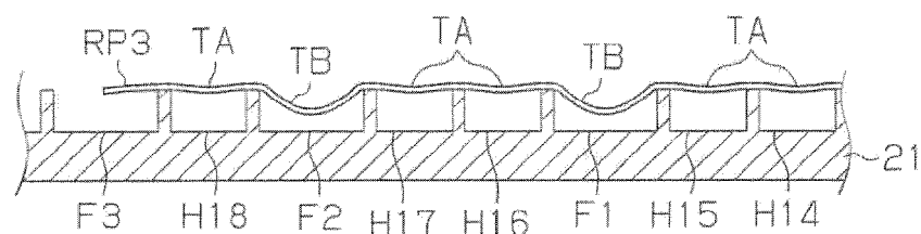
Fig. 4C (Prior Art)
