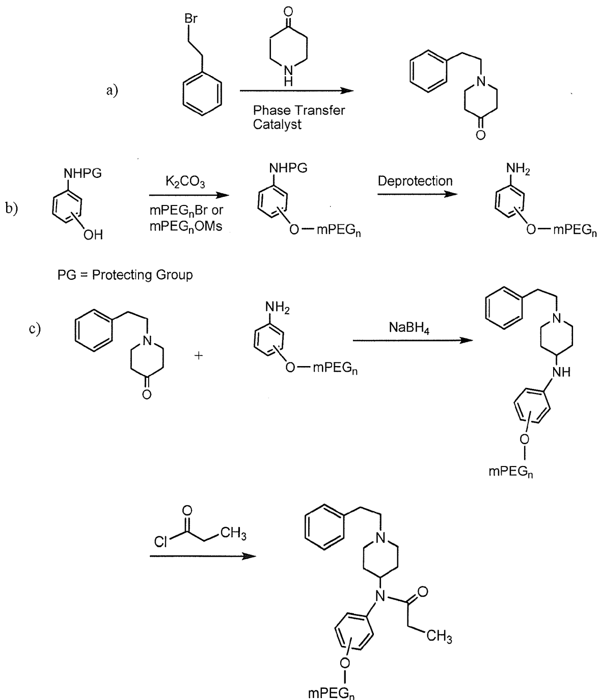
Scheme 11-C
