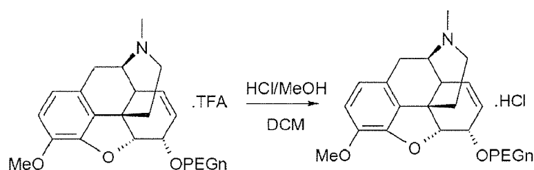
Compound B
