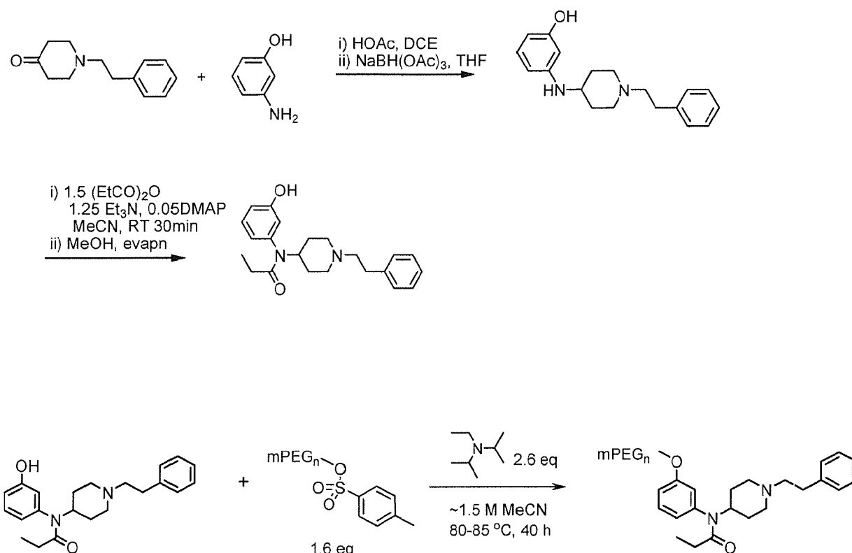
Scheme 11-D
