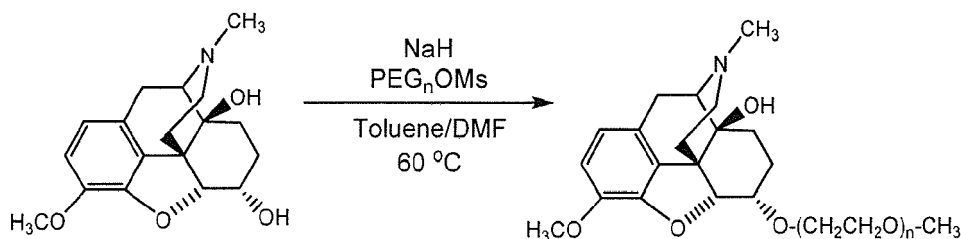
Compound C
