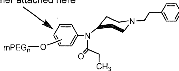
Scheme 11-C
