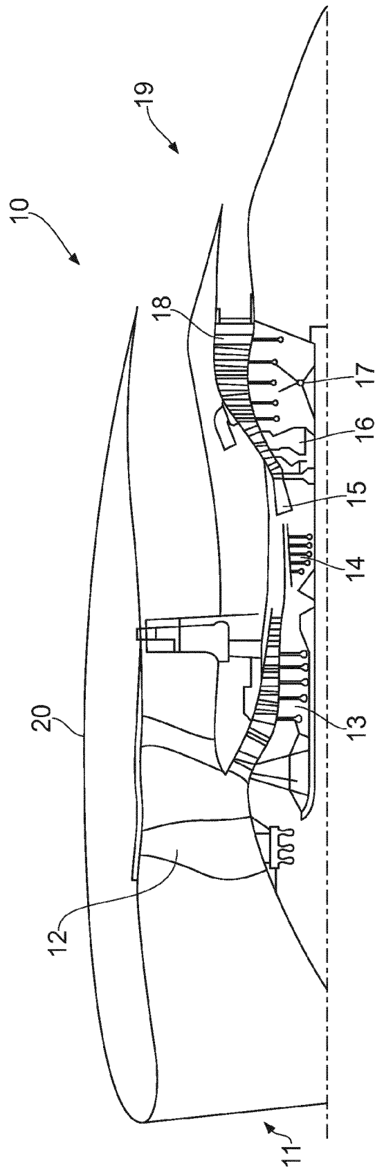
FIG. 2 (Prior Art)
