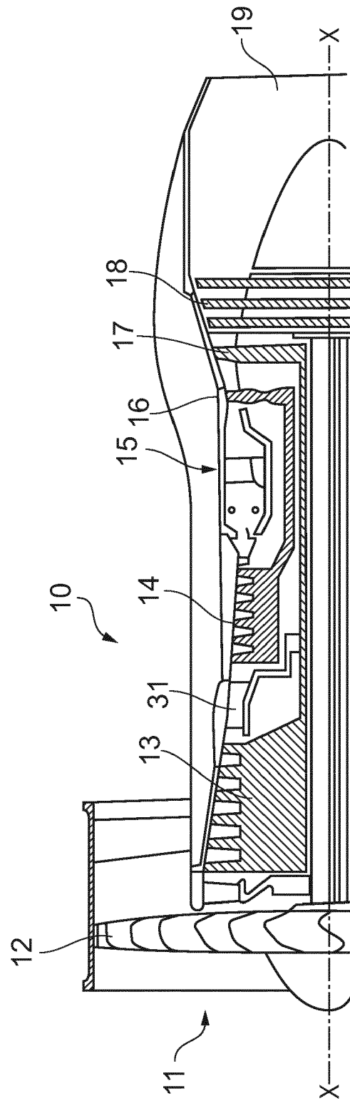
FIG. 1 (Prior Art)
