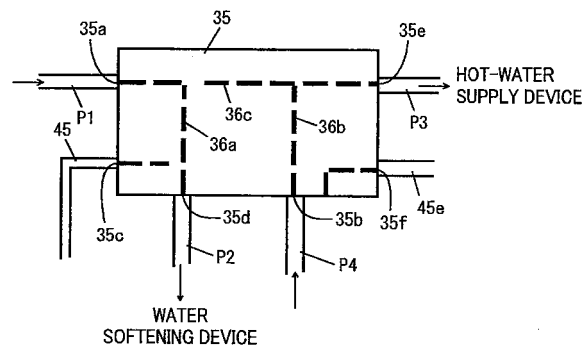
FIG.4B SECOND POSITION
