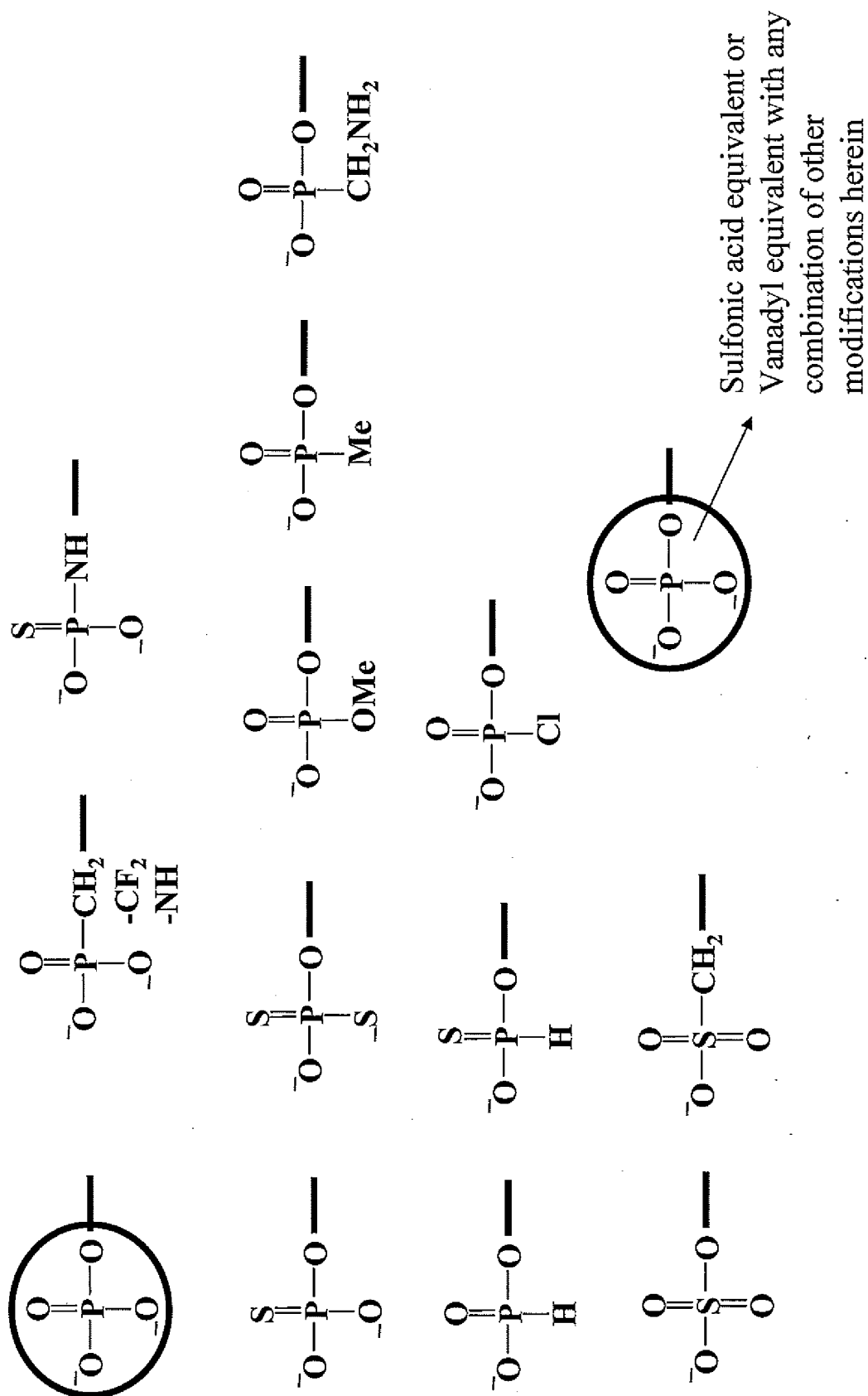
Figure 8: 5'-phosphate modifications
