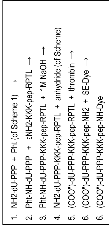
Scheme 10 - g-dNTP With Carboxylated Base
