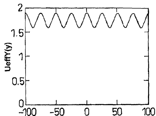
M = 2000 at rf plates 0.3V ripple
