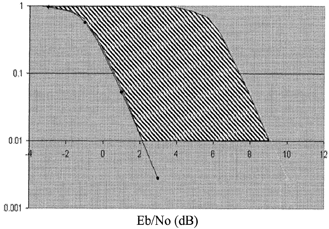
FER over various codecs d1/d2=3 dB TU50
