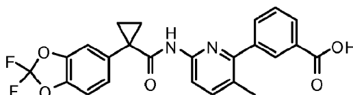
Compound 1.
