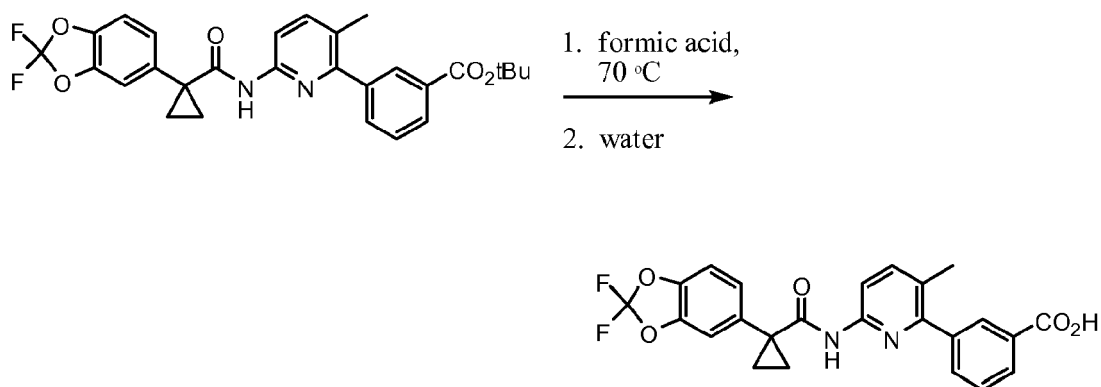
Compound 1
