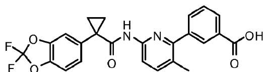
Compound 1
