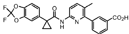
Compound 1
