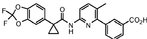
Compound 1.
