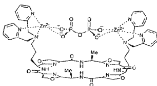
compound 5
