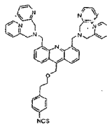
compound 8
