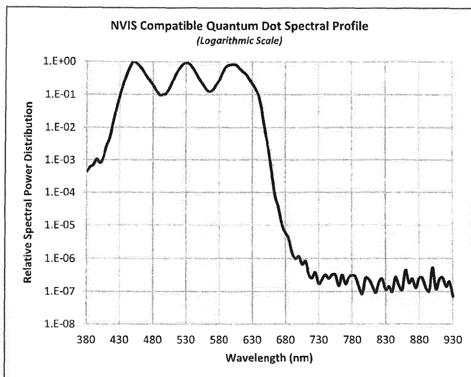
Figure 4. Spectral profile of LCD-based display utilizing NVIS-compatible photoluminescent backlight.
