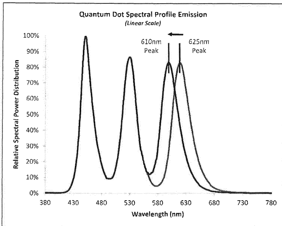
Figure 3. Shifted long-wavelength peak of an NVIS-compatible backlight utilizing the layer of photoluminescent material.
