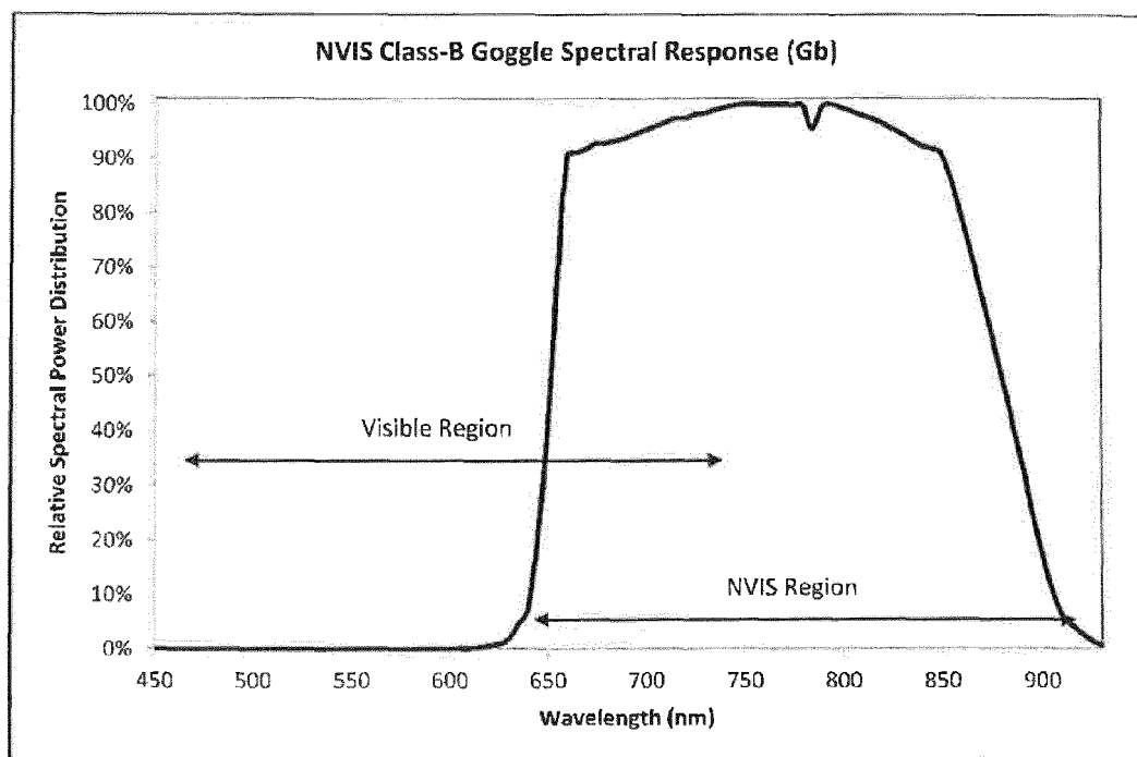
Figure 1. Class-B NVIS goggles spectral response
