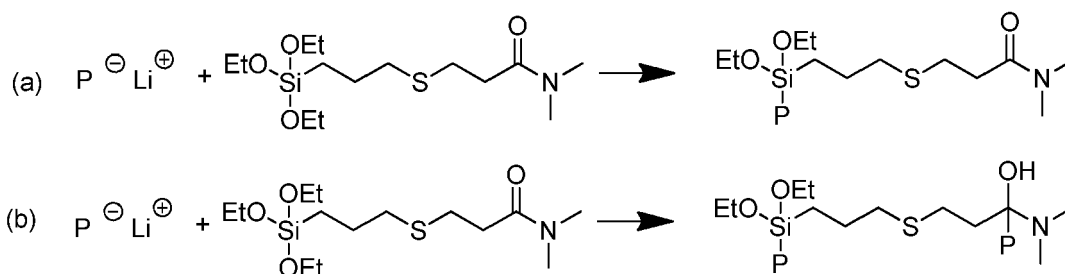
Scheme 1 Theorized mechanism of action of siloxy acrylamide end terminating agent
