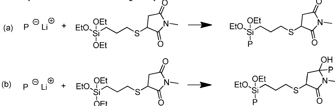
Scheme 2 Theorized mechanism of action of siloxy maleimide end terminating agent
