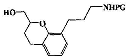
T100a [(R)-isomer] T100b [(S)-isomer]
