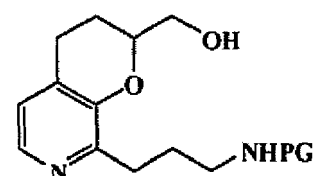
T131a [(R)-isomer] T131b [(S)-isomer]
