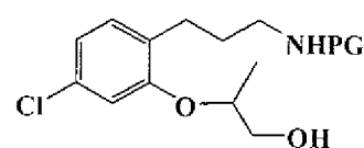
T111a [(R)-isomer] T111b [(S)-isomer]
