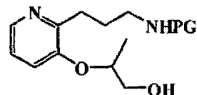
T103a [(R)-isomer] T103b [(S)-isomer]
