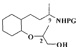
T130a [(2R,9R)-isomer] T130b [(2S,9S)-isomer] T130c [(2R,9S)-isomer] T130d [(2S,9R)-isomer]
