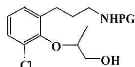
T115a [(R)-isomer] T115b [(S)-isomer]
