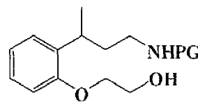
T39a [(R)-isomer] T39b [(S)-isomer]
