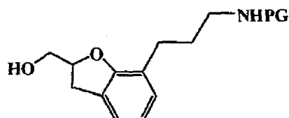
T105a [(R)-isomer] T105b [(S)-isomer]
