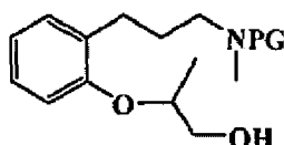
T122a [(R)-isomer] T122b [(S)-isomer]
