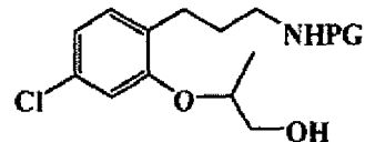
T111a [(R)-isomer] T111b [(S)-isomer]
