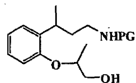
T118a [(2R,7R)-isomer] T118b [(2S,7S)-isomer] T118c [(2R,7S)-isomer] T118d [(2S,7R)-isomer]
