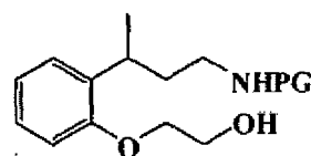
T39a [(R)-isomer] T39b [(S)-isomer]
