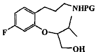
T116a [(R)-isomer] T116b [(S)-isomer]
