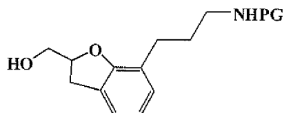
T105a [(R)-isomer] T105b [(S)-isomer]
