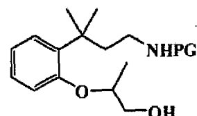
T123a [(R)-isomer] T123b [(S)-isomer]
