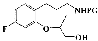
T75a [(R)-isomer] T75b [(S)-isomer]
