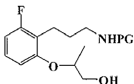
T110a [(R)-isomer] T110b [(S)-isomer]
