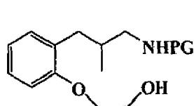
T40a [(R)-isomer] T40b [(S)-isomer]
