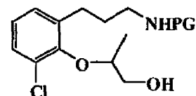
T115a [(R)-isomer] T115b [(S)-isomer]
