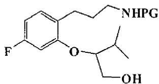
T116a [(R)-isomer] T116b [(S)-isomer]
