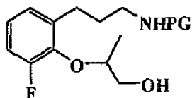
T109a [(R)-isomer] T109b [(S)-isomer]
