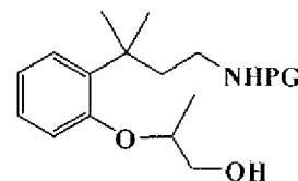
T123a [(R)-isomer] T123b [(S)-isomer]
