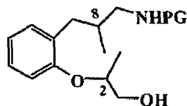
T114a [(2R,8R)-isomer] T114b [(2S,8S)-isomer] T114c [(2R,8S)-isomer] T114d [(2S,8R)-isomer]
