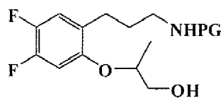
T112a [(R)-isomer] T112b [(S)-isomer]
