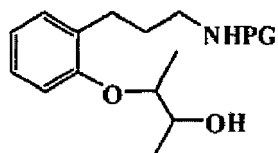
T124a [(1R,2R)-isomer] T124b [(1S,2S)-isomer] T124c [(1R,2S)-isomer] T124d [(1S,2R)-isomer]
