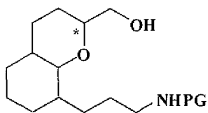
T132a [(R*)-isomer] T132b [(S*)-isomer]
