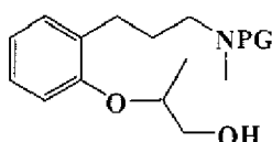
T122a [(R)-isomer] T122b [(S)-isomer]
