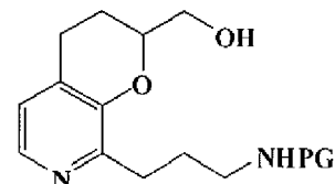
T131a [(R)-isomer] T131b [(S)-isomer]
