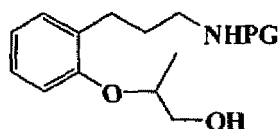
T33a [(R)-isomer] T33b [(S)-isomer]
