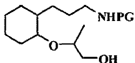
T102a [(R)-isomer] T102b [(S)-isomer]
