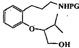
T117a [(R)-isomer] T117b [(S)-isomer]
