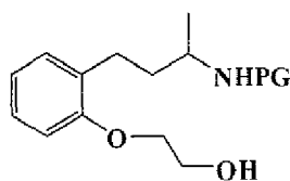
T125a [(R)-isomer] T125b [(S)-isomer]
