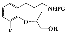
T109a [(R)-isomer] T109b [(S)-isomer]
