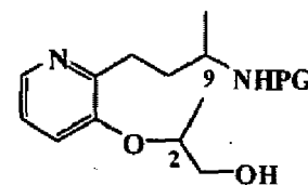
T126a [(2R,9R)-isomer] T126b [(2S,9S)-isomer] T126c [(2R,9S)-isomer] T126d [(2S,9R)-isomer]
