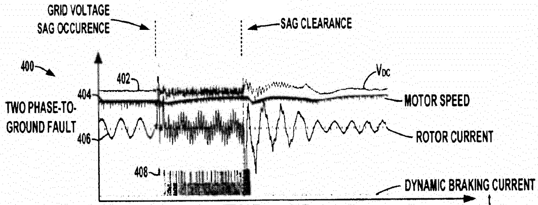
FIG. 12 (PRIOR ART)
