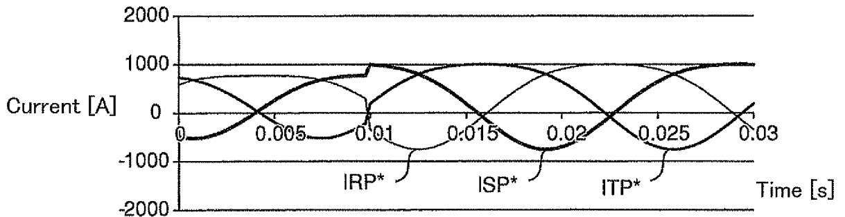
FIG.38D Upper valve branch current reference value — I_{RP}^* — I_{SP}^* — I_{TP}^*
