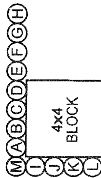
(a) Intra_4x4
