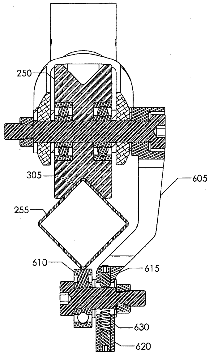
SECTION M-M
