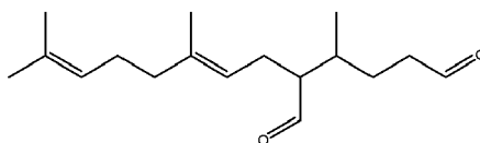
(b3)
