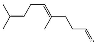
(C11 aldehyde 1)
