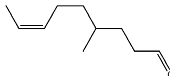
(C11 aldehyde 2)
