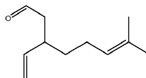
(C11 aldehyde 4)
