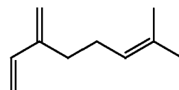
(f) 7-methyl-3-methyleneocta-1,6-diene COMMON NAME: Beta-Myrcene
