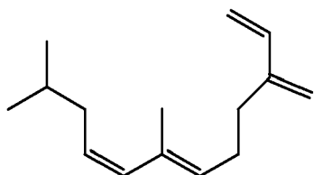
(e) (6E,8Z)-7,11-dimethyl-3-methylenedodeca-1,6,8-triene
