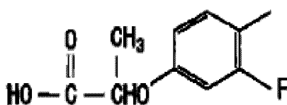
(IX)
