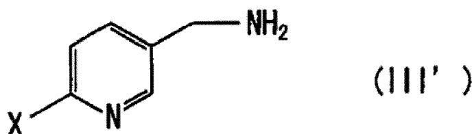
[Chemical Formula 17]
