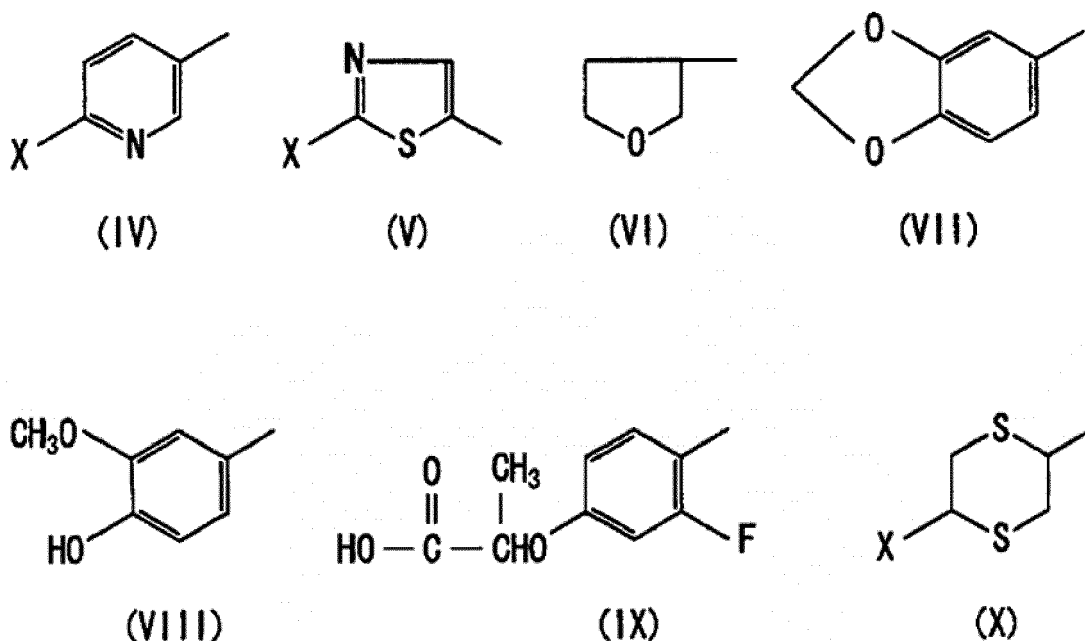
[Chemical Formula 4]
