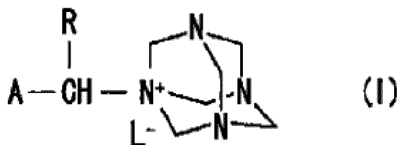
[Chemical Formula 1]
