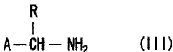
[Chemical Formula 3]
