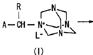
[Chemical Formula 1]
