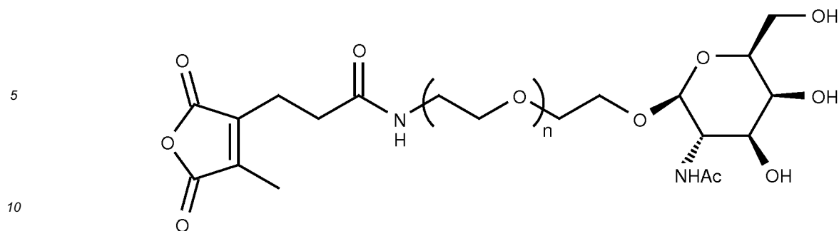
CDM-NAG
