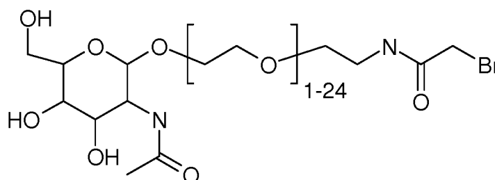
N-NAG-PEG bromo acetimide
