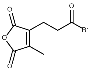
CDM
