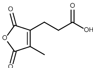
CDM
