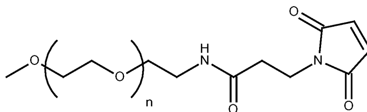
PEG maleimide
