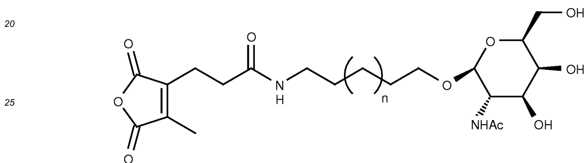
CDM-NAG (alkyl spacer)
