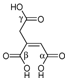
aconitic acid
