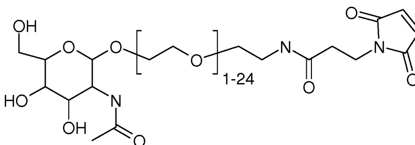
NAG-PEG maleimide
