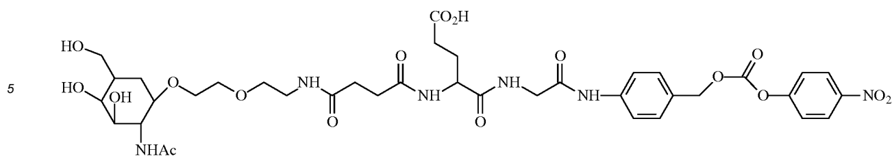
NAG-Glu-Gly-PABC-PNP
