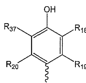
(IVc)
