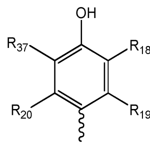
(IVc)
