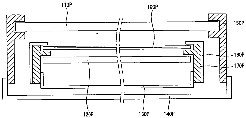
FIG. 1 (RELATED ART)
