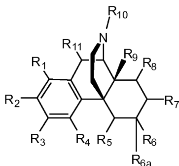
Formula I(c)
