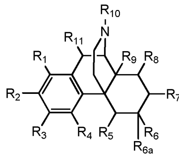
Formula I(f)
