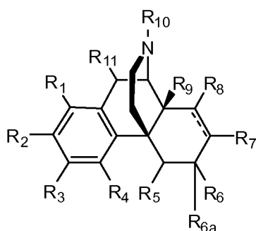
Formula (Ia)
