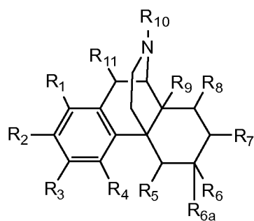
Formula I(e)
