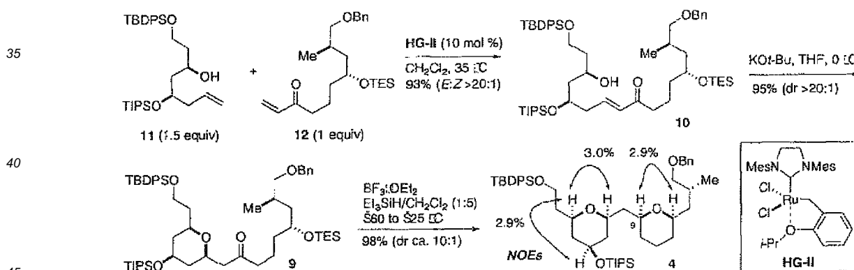
Scheme 4. Synthesis of methylene bis(tetrahydropyran) 4.
