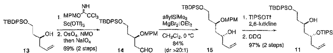
Scheme 2. Synthesis of hydroxy olefin 11.
