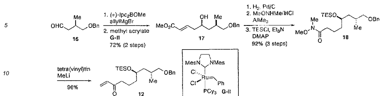
Scheme 3. Synthesis of enone 12.
