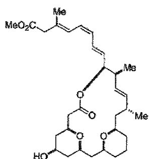
Analog 1 (HF27155)
