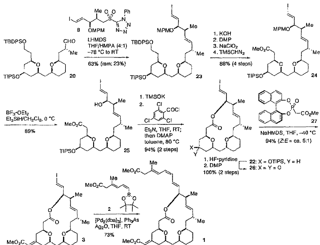
Scheme 6. Completion of the total synthesis.
