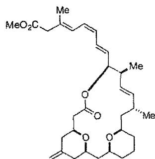
Analog 8 (HF27191)
