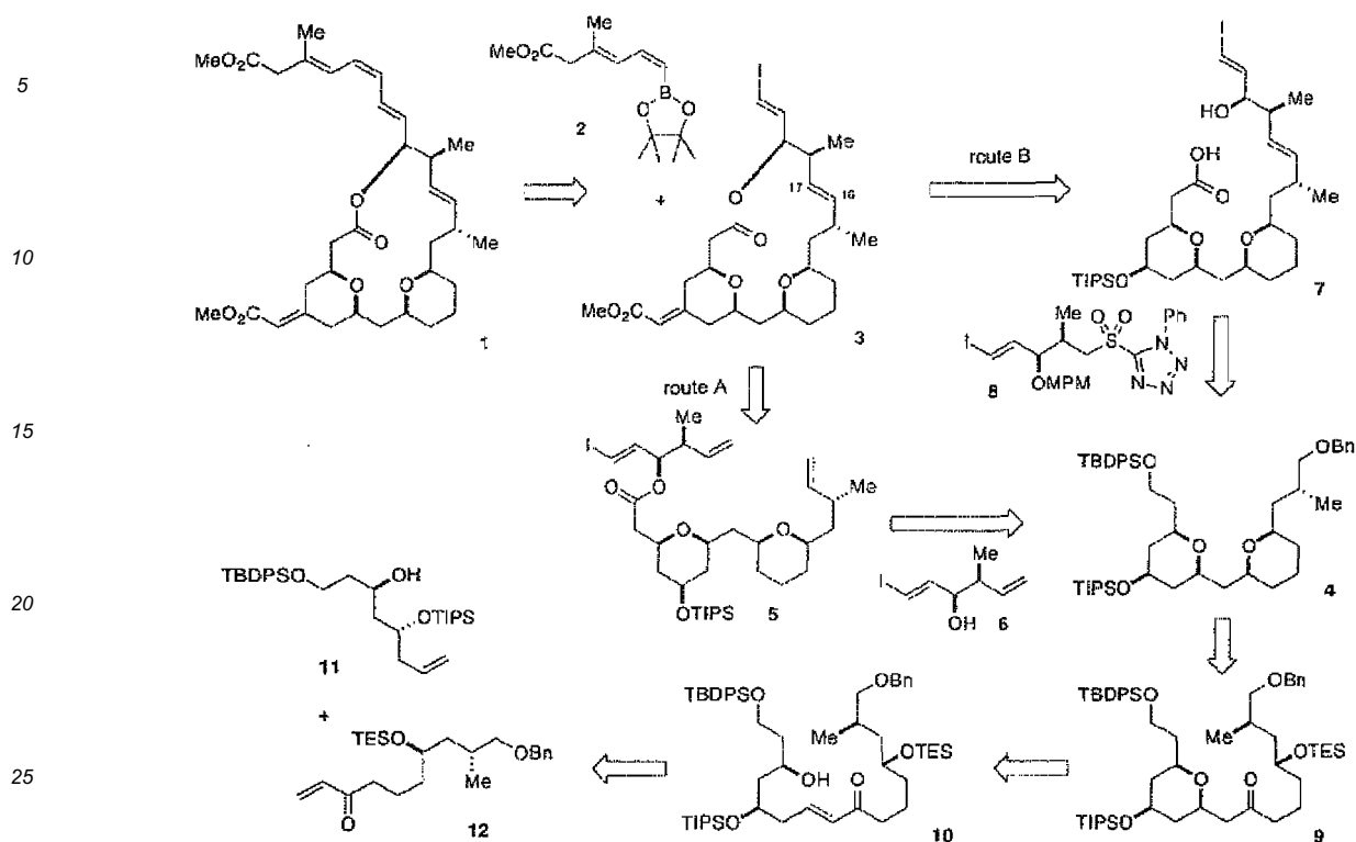
Scheme 1. Synthetic plan toward (-)-exiguolide (1).
