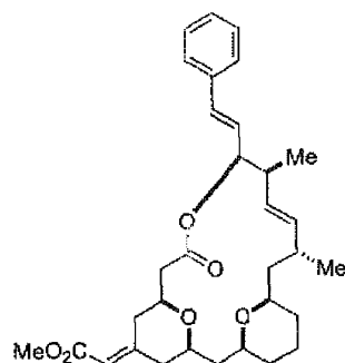
Analog 5 (HF27189)
