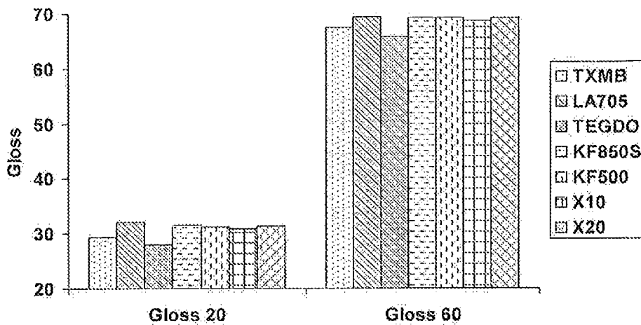
Figure 7. Gloss of Acrylic Semigloss Formulations
