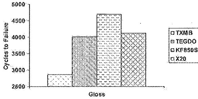
Figure 11. Acrylic Copolymer Gloss Scrub Resistance
