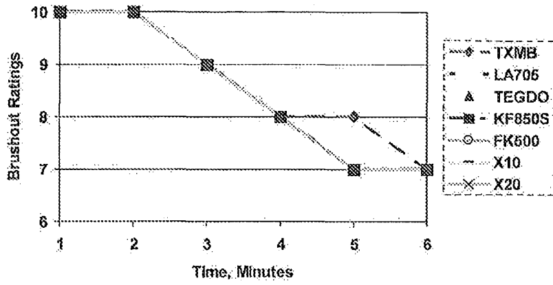
Figure 5. Acrylic Semigloss Wet Edge/Open Time Ratings
