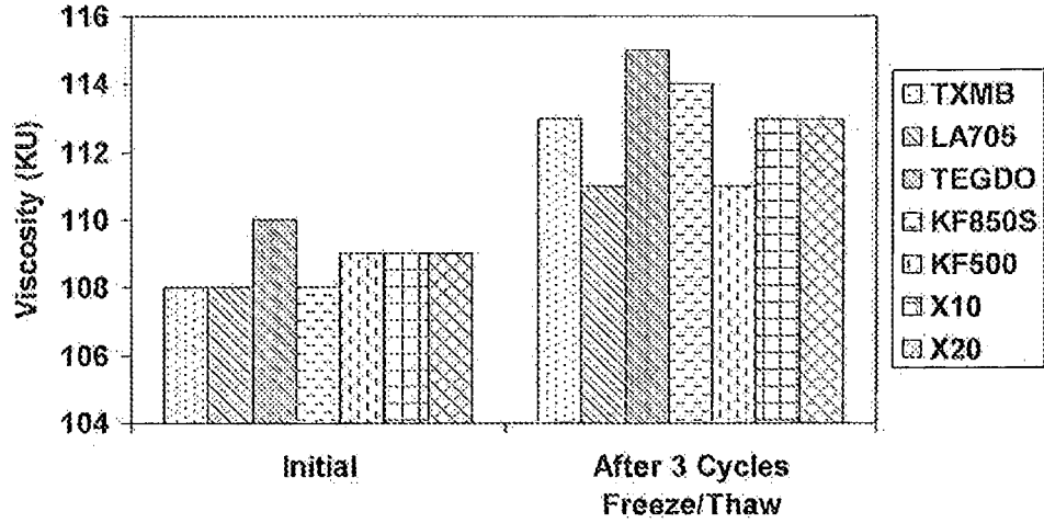
Figure 3. Acrylic Semigloss Viscosity Stability After Three Cycles of Freeze/Thaw
