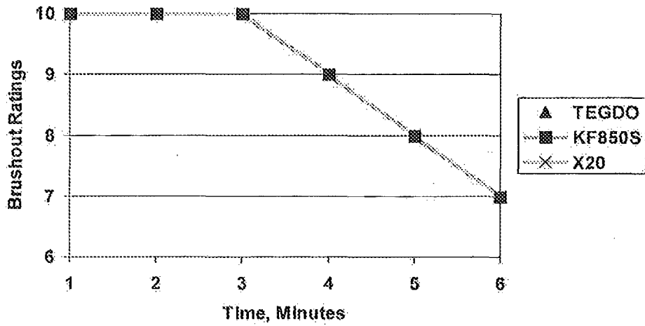
Figure 6. Acrylic Copolymer Gloss Wet Edge/Open Time Ratings
