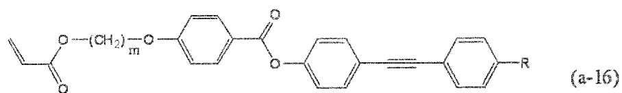
[Chem. 26]
