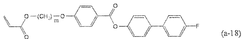
[Chem. 28]
