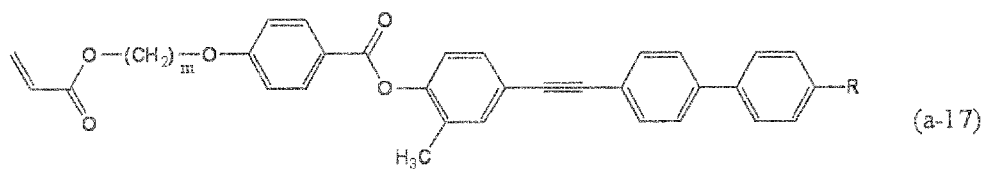
[Chem. 27]
