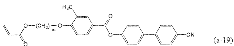
[Chem. 29]
