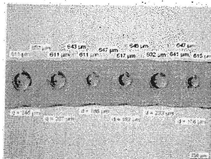
Fig. 9b Inventive reinforced film 2 (Middle)
