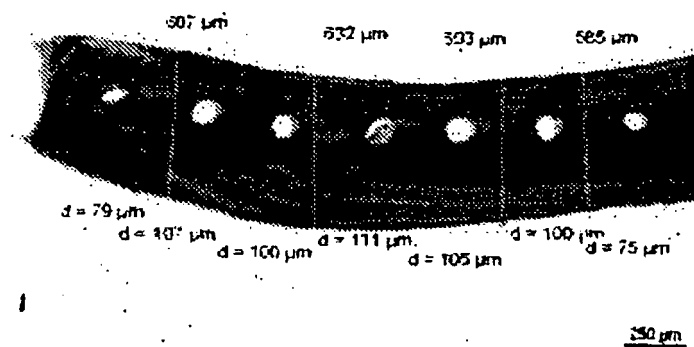
Fig. 12a Comparative film C (Initial End)
