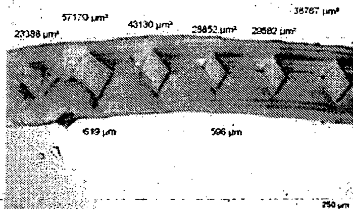
Fig. 8b Inventive reinforced film 1 (Terminal End)
