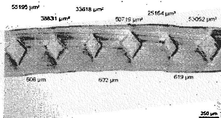
Fig. 8a Inventive reinforced film 1 (Initial End)
