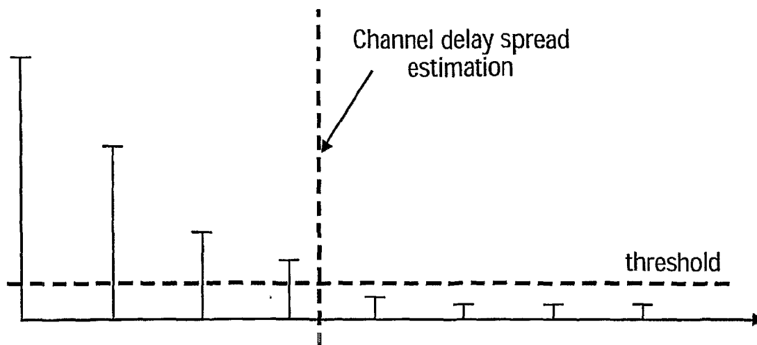
a) Threshold technique for adaptive LS with smoothing
