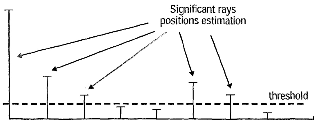
b) Threshold technique for adaptive ML
