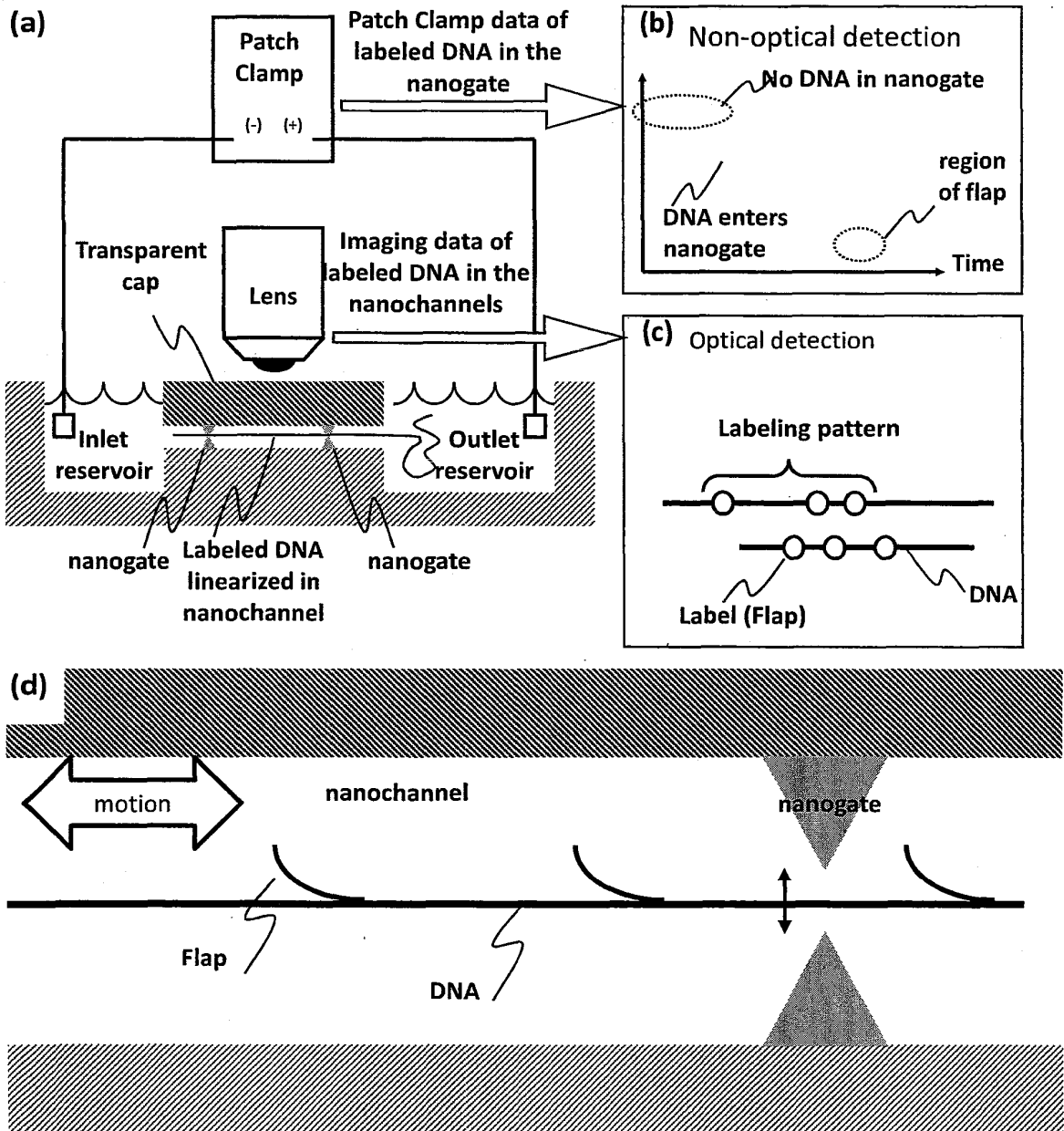
FIG 8: Optical and non-optical detection schemes
