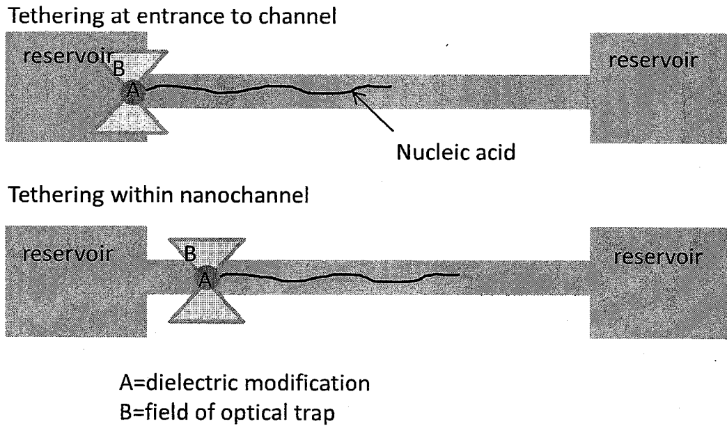
Fig 11 b : Optical trapping for tethering nucleic acid
