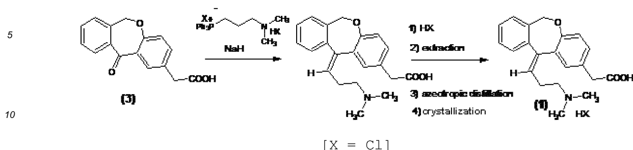
Reaction scheme 3
