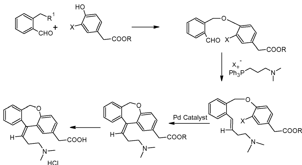
Reaction scheme 2
