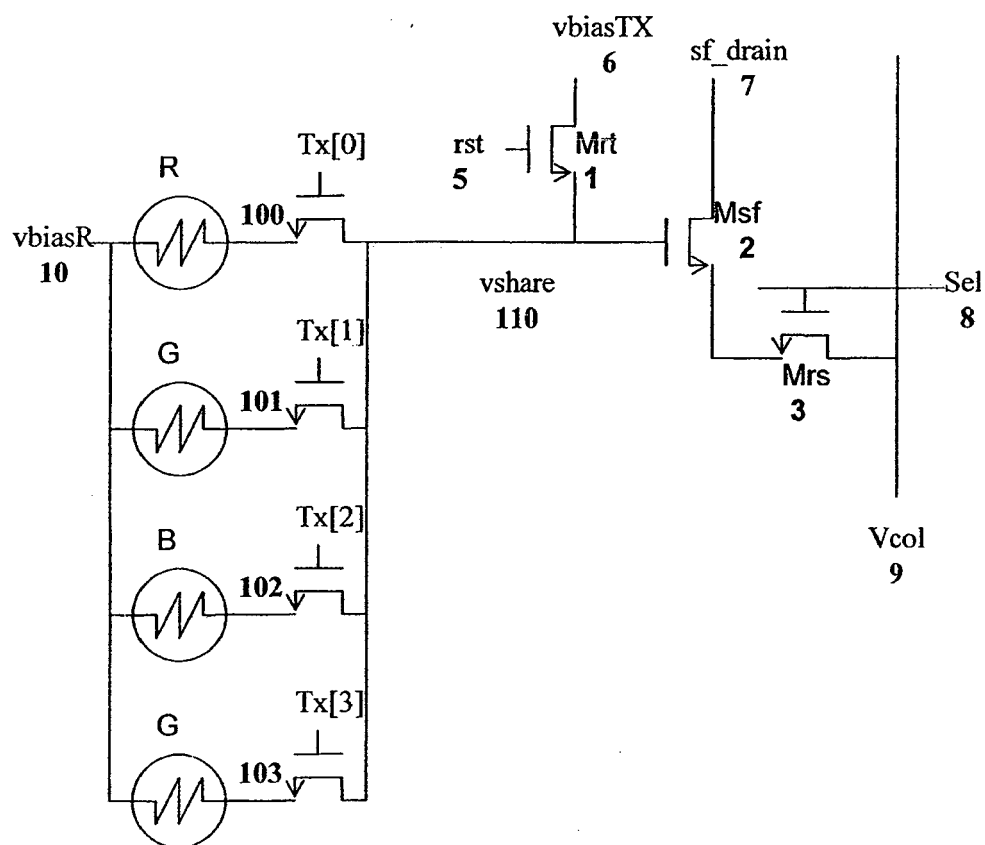
Schematic for 3T-1.1um Pixel with 4-to-1 sharing
