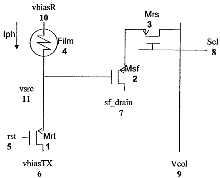
Schematic for 3T 2.4um Pixel - PMOS
