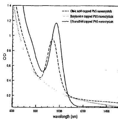
(a) Absorption spectrophotometry
