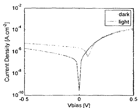
Figure 57. Steady-state I - V characteristics in the dark and at 17.9 \mu\text{W.cm}^{-2} illumination at 1550 nm.
