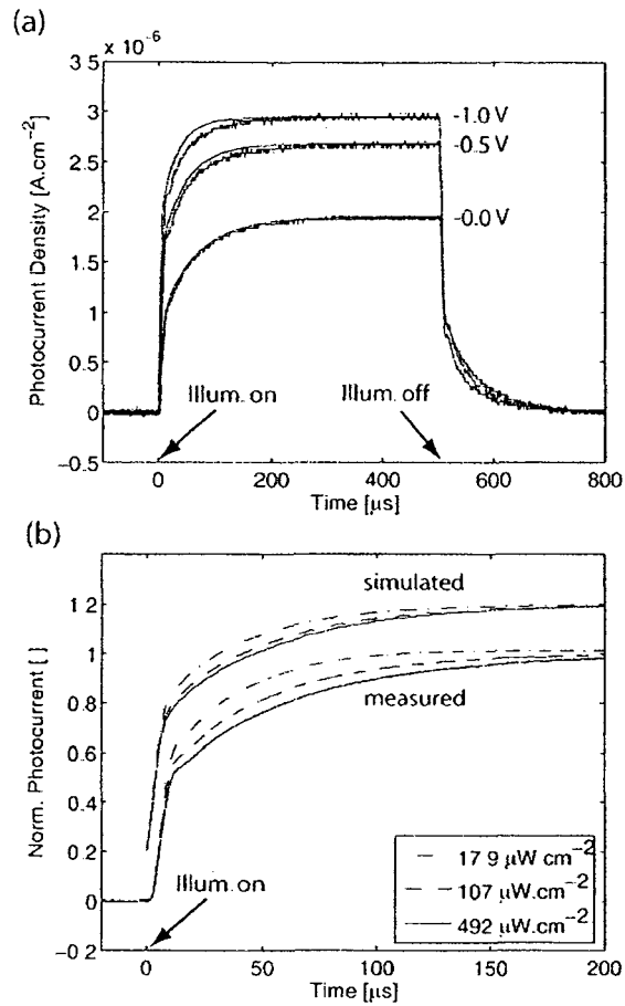
Figure 56. (a) Measured (noisy line) and simulated (smooth line) photocurrent transient response as a function of bias to a square illumination pulse at 17.9 \mu\text{W} \cdot \text{cm}^{-2} . Note that the measured and simulated lines are co-incident for 0.0V. (b) Measured and simulated photocurrent transient response (normalized) as a function of irradiance at zero bias. The simulated response is shifted for clarity.
