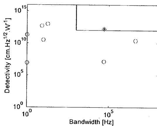
Figure 52. Detectivity and bandwidth of previously reported solution-processed photodetectors (circles), and the photodetector presented in our submission (star).
