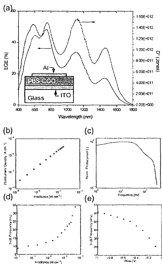
Figure 53. (a) External quantum efficiency (at 295 K) and normalized detectivity (at 250 K) as a function of wavelength. The inset shows a schematic representation of the photodiode device architecture. (b) Photocurrent density as a function of irradiance at 1550 nm. (c) Frequency dependence of photocurrent at zero bias and 17.9 \mu W \cdot cm^{-2} irradiance and 3dB frequency dependence on irradiance (d) and bias (e).
