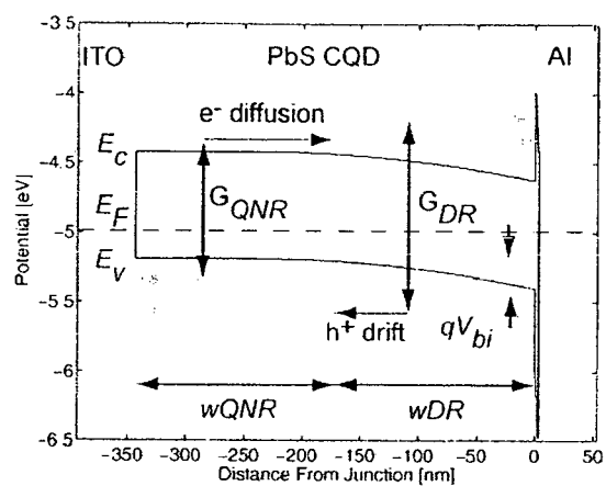
Figure 55. Energy bands and photocurrent components in the quasi-neutral and depletion regions of photodiode.
