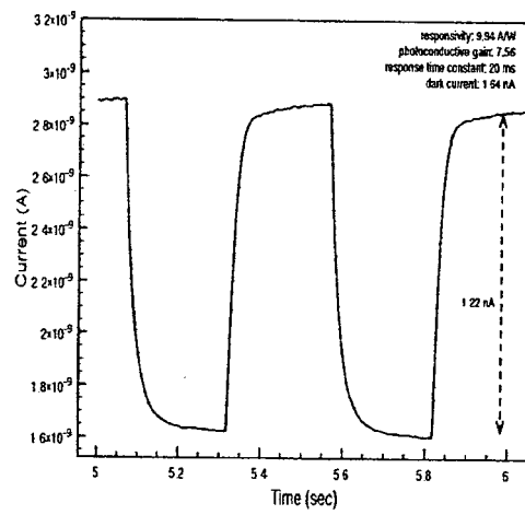
(a) Typical transient response
